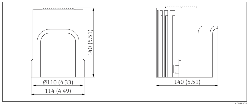
33 Dimensions of weather protection cover PBT. Unit of measurement mm (in)
