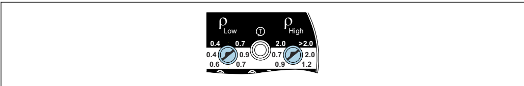
33 Density setting for maximum detection for media such as liquefied gas
