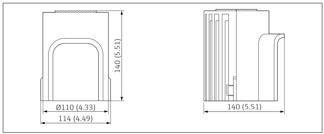
47 Dimensions of weather protection cover PBT. Unit of measurement mm (in)
