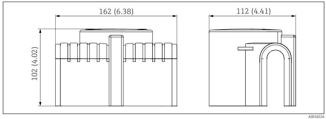
46 Dimensions of weather protection cover PA6. Unit of measurement mm (in)
