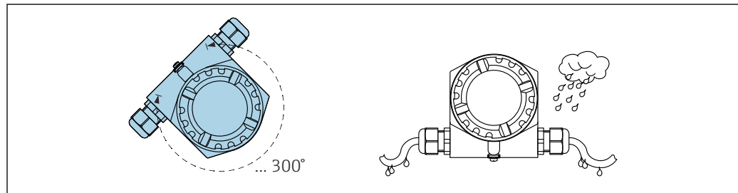
17 Housing without set screw; form a drip loop on the cable
