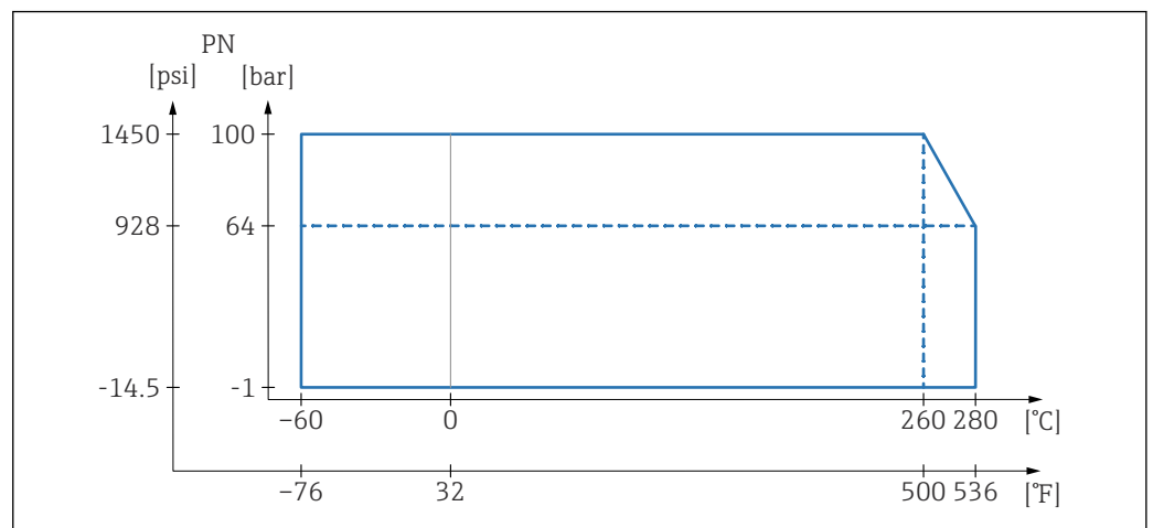
54 Process pressure range for high-temperature version with 230 °C (450 °F)/280 °C (540 °F)
