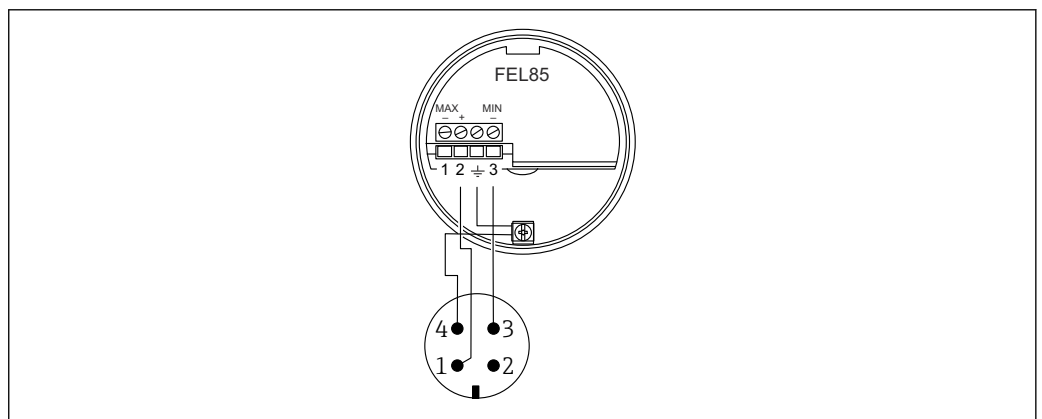
20 Terminal assignment with M12 connector, minimum detection mode of operation
