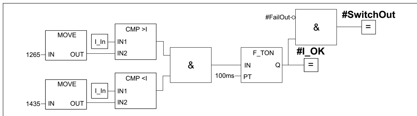
27 Function block, switch output
