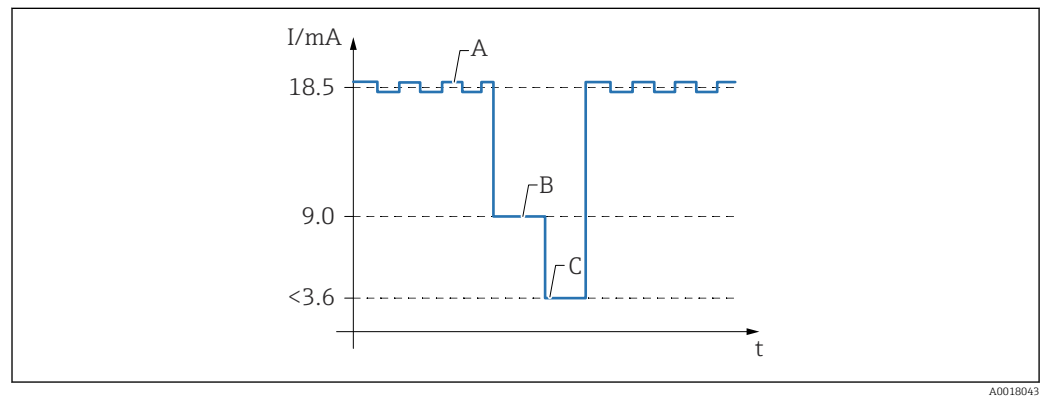
36 Proof testing procedure for minimum detection
