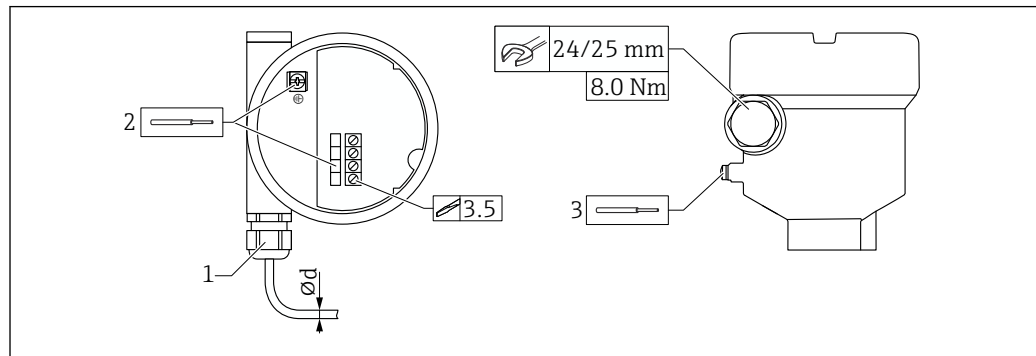
21 Example of coupling with cable entry, electronic insert with terminals
