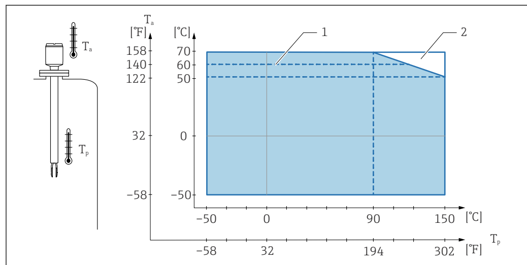
51 Permitted ambient temperature T_a at the housing as a function of the process temperature T_p in the vessel; maximum process temperature 150 °C (302 °F)
