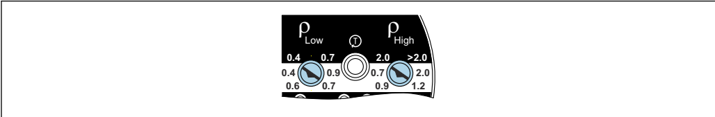
30 Density setting for minimum detection for media such as alcohol
