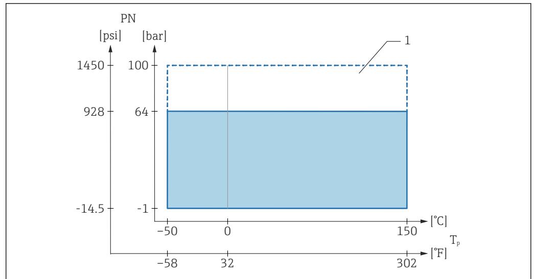
53 Process pressure range at process temperature T_p to 150 °C (300 °F)
