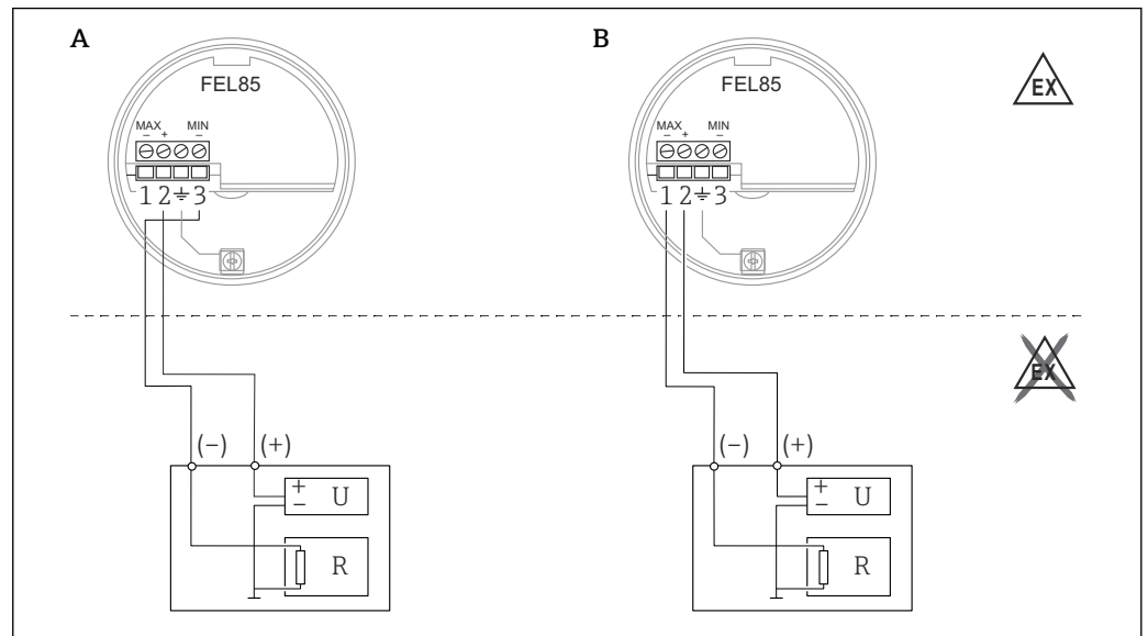
22 Connecting to a PLC
