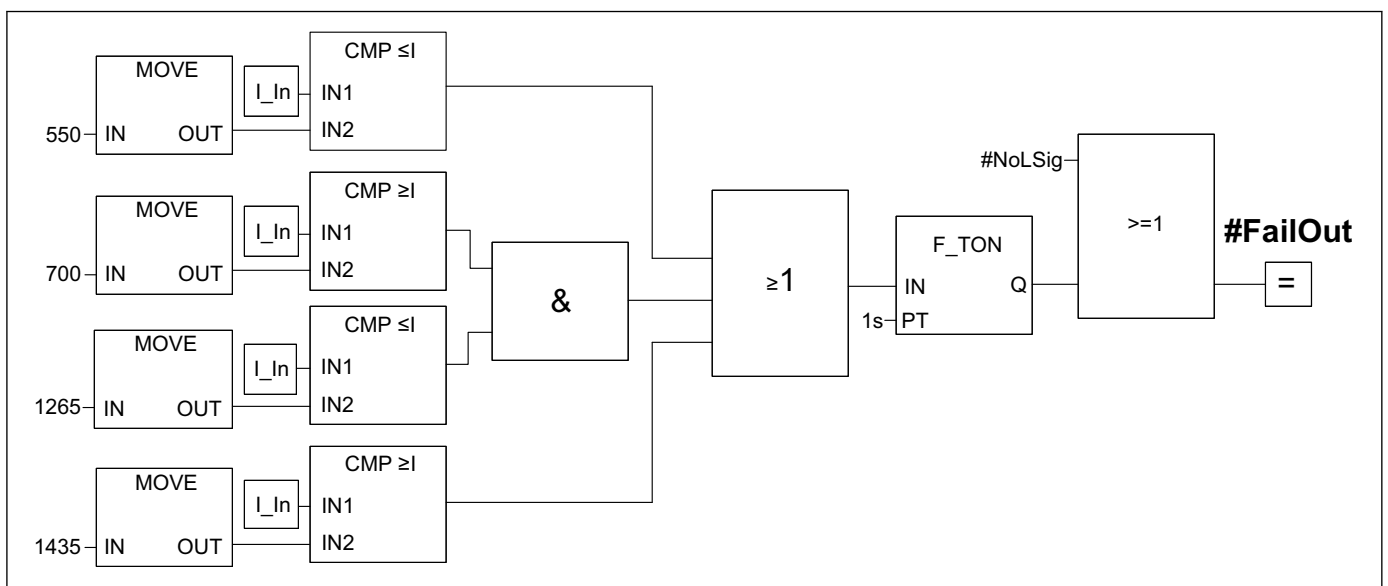
26 Function block, error current analysis
