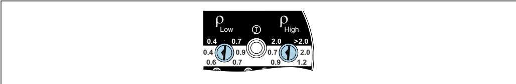
29 Density setting for minimum detection for media such as liquefied gas
