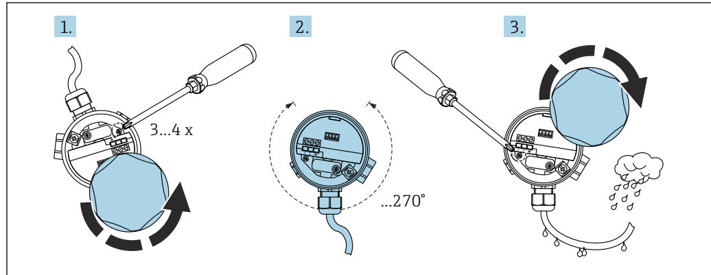
16 Housing with locking screw; form a drip loop on the cable
