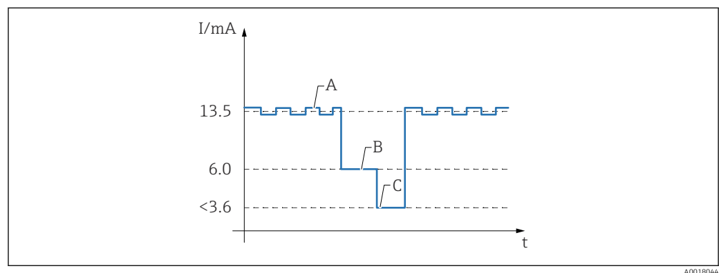
37 Proof testing procedure for maximum detection
