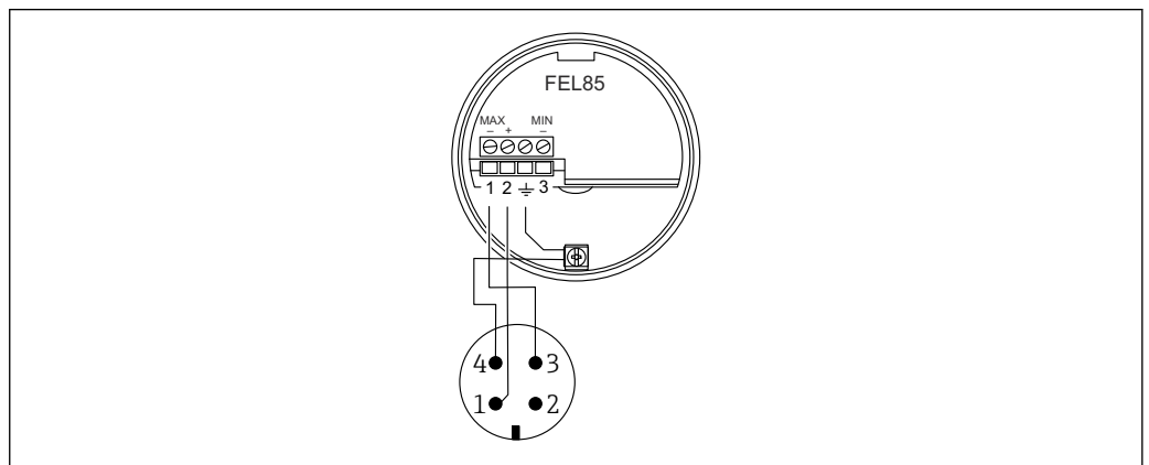
19 Terminal assignment with M12 connector, maximum detection mode of operation
