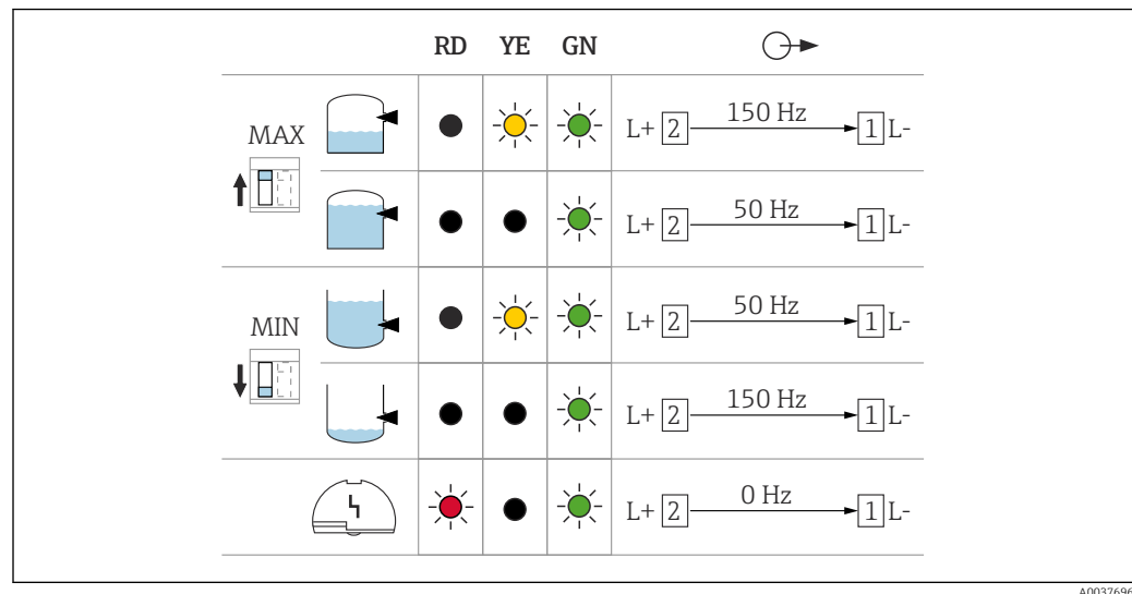
28 Switching behavior and signaling, electronic insert FEL67
