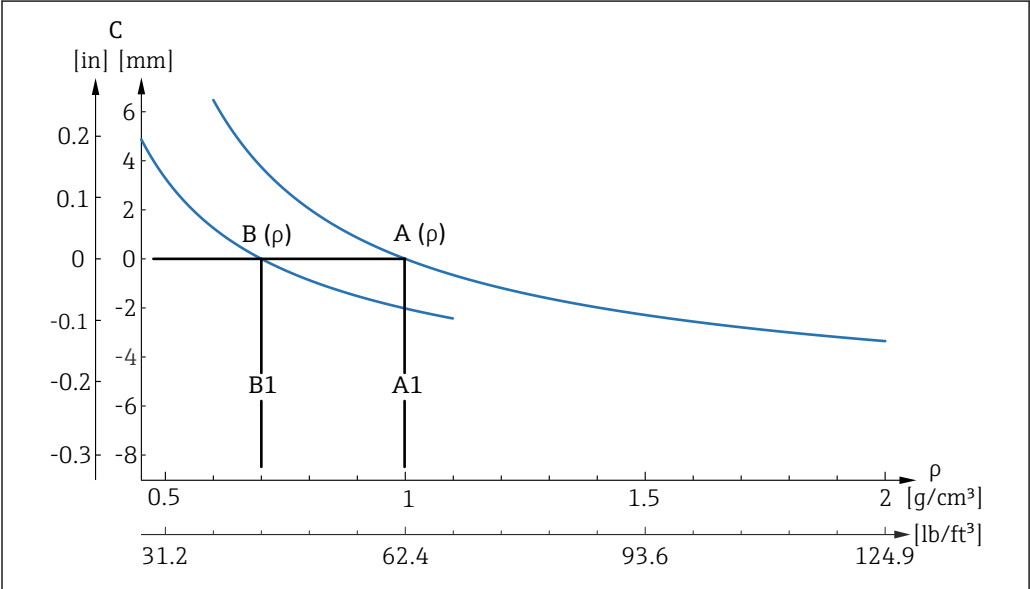
9 Switch point deviation over density, 316L A Density switch setting ( \rho > 0.7 g/cm 3 (43.7 lb/ft 3 )) A1 Reference operating condition \rho = 1 g/cm 3 (62.4 lb/ft 3 ) B Density switch setting ( \rho > 0.5 g/cm 3 (31.21 lb/ft 3 )) B1 Reference operating condition \rho = 0.7 g/cm 3 (43.7 lb/ft 3 ) C Switch point deviation
