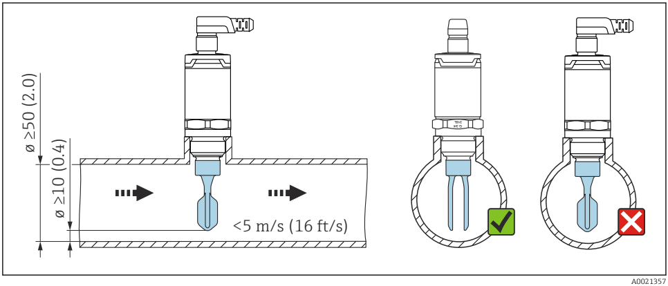
8 Position of the tuning fork in pipes. Unit of measurement mm (in)
