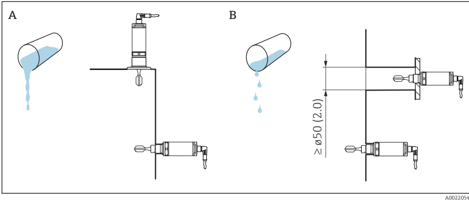
4 Installation options with consideration given to the liquid viscosity, dimensions in mm (in)
