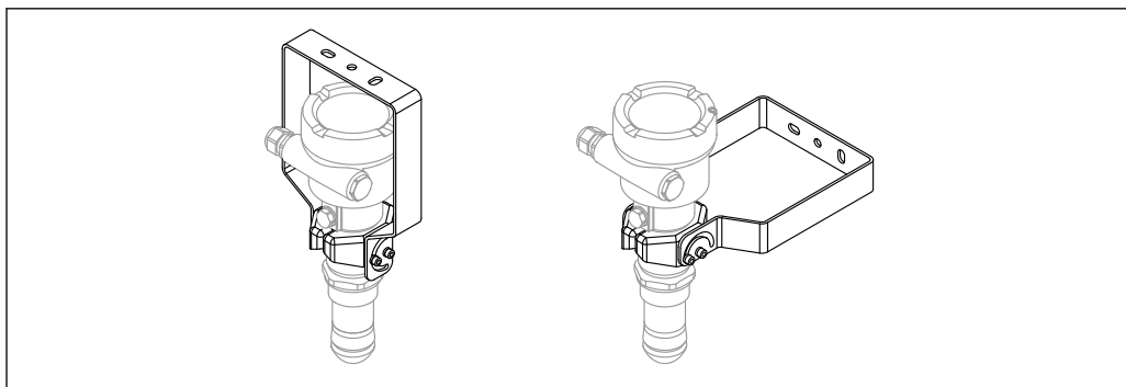
43 Mounting bracket adjustable FMR6xB; ceiling or wall mounting
