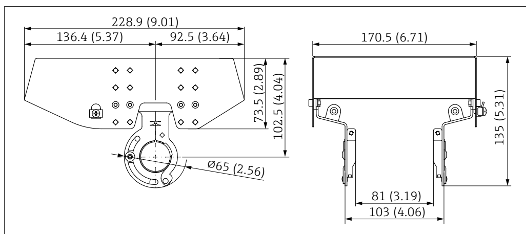
41 Dimensions of weather protection cover, 316 L, XW112. Unit of measurement mm (in)
