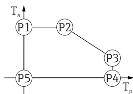
13 Plastic housing; process temperature 0 to +130 °C (+32 to +266 °F) with CSA C/US approval
