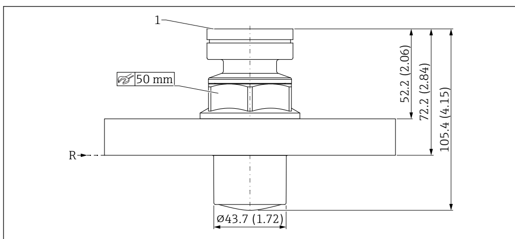
27 Dimensions of encapsulated antenna, PVDF, 40 mm (1.5 in), process connection UNI flange. Unit of measurement mm (in)
