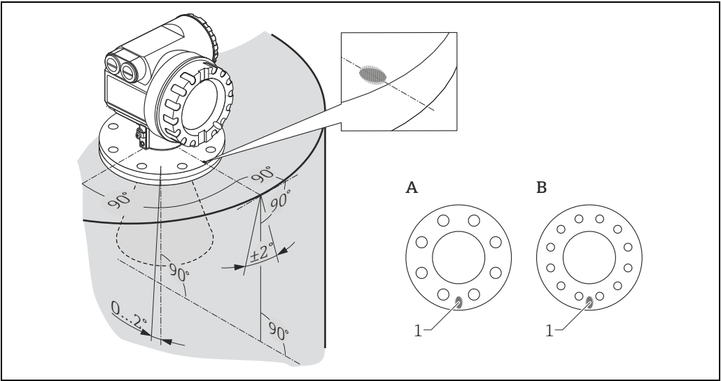
1 Markings on device flange A DN 150, ANSI 6" B DN 200 to 250, ANSI 8" to 10"
