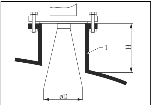
1 Nozzle
