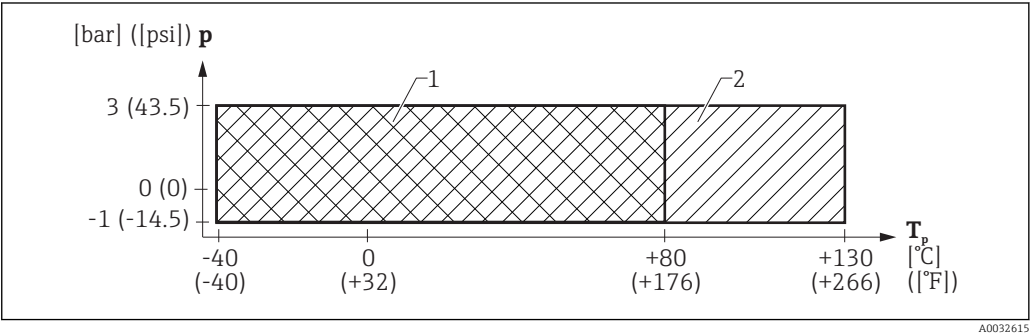
26 FMR50: Permitted range for process temperature and process pressure
