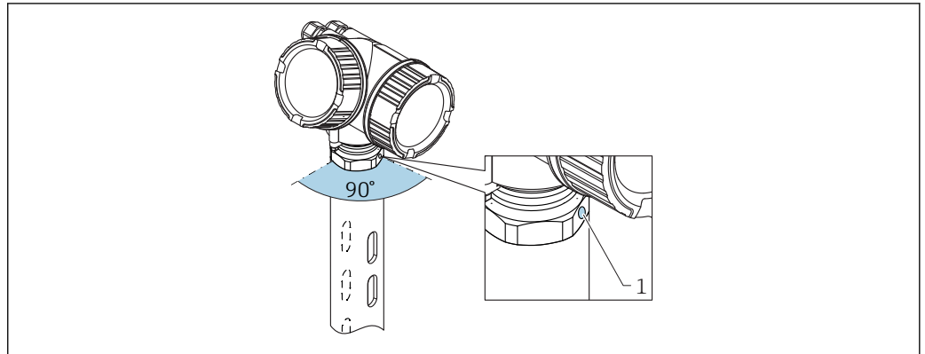
■ 24 Installation in stilling well
