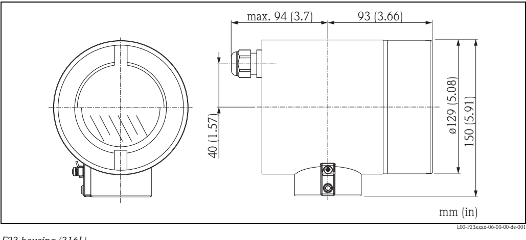
F23 housing (316L)
