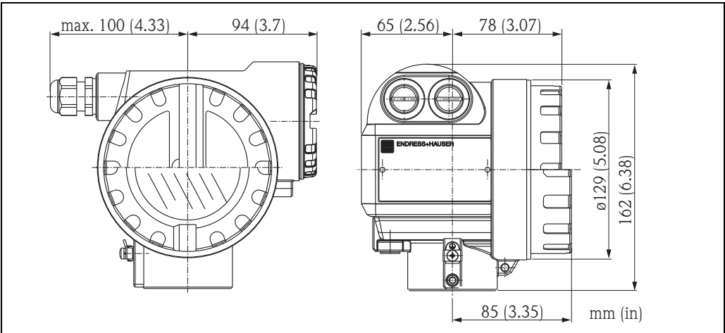
T12 housing (Aluminium)
