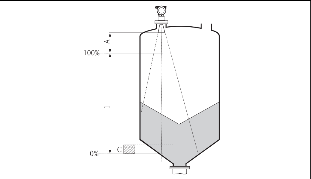
1 Measuring range
