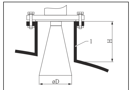
1 Nozzle
