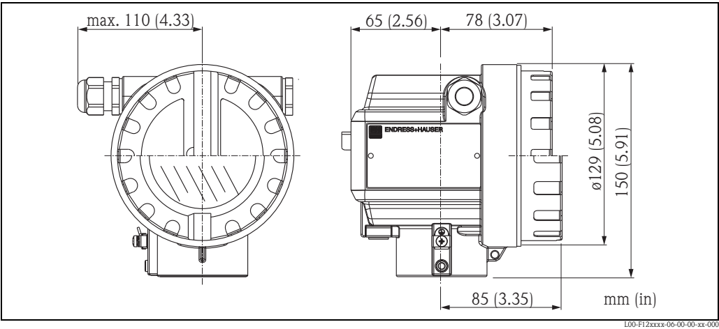
F12 housing (Aluminium)
