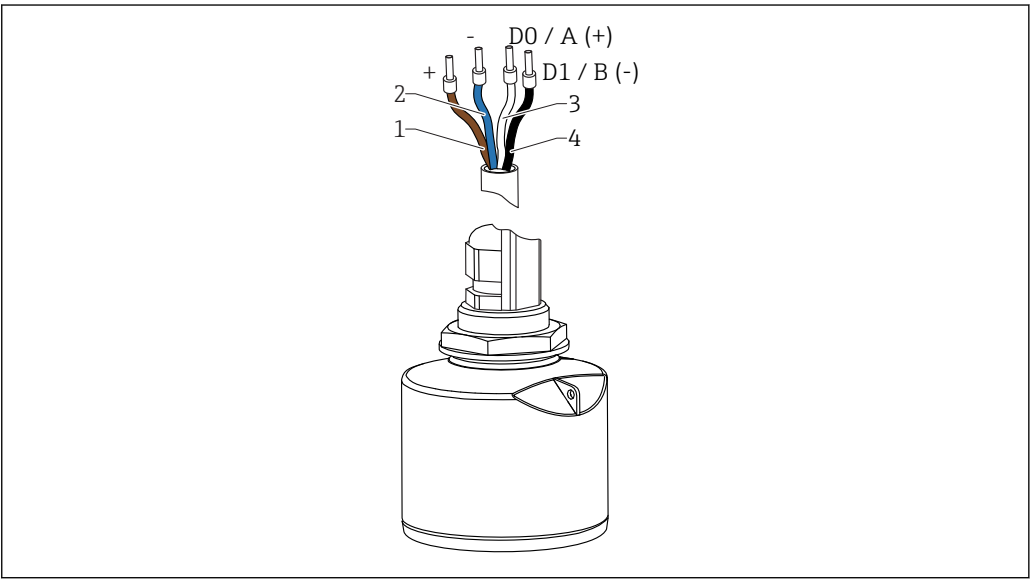
2 FMR20 cable assignment, Modbus
