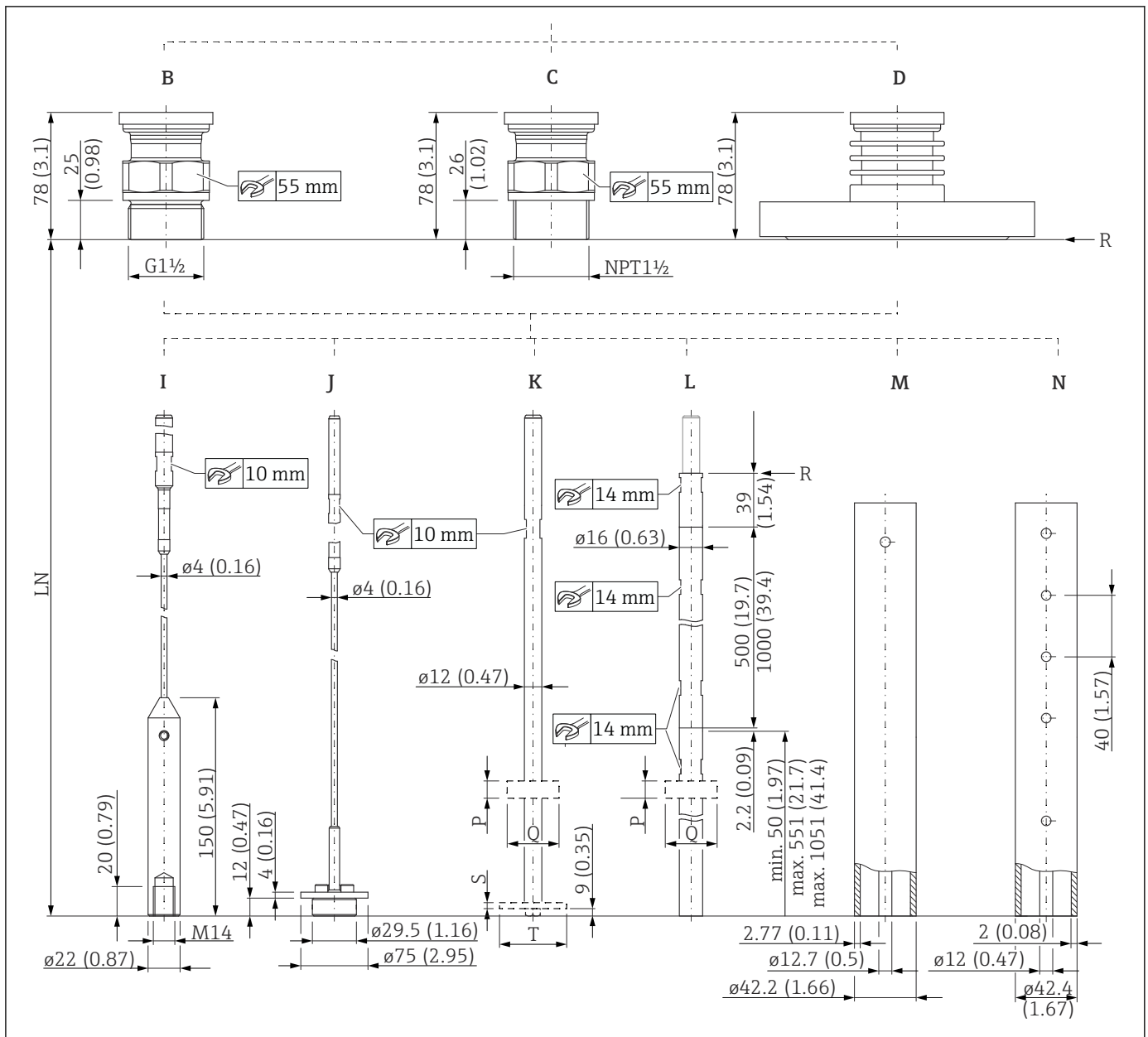
48 FMP51: Process connection/probe. Unit of measurement mm (in)
