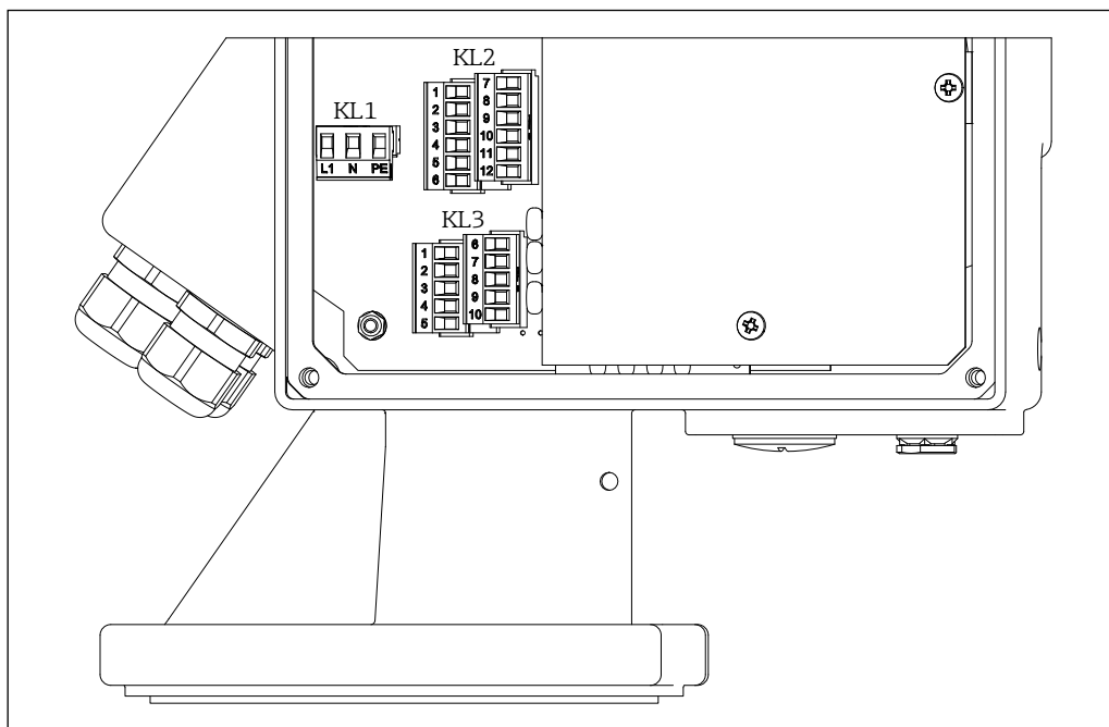
4 Terminal assignment
