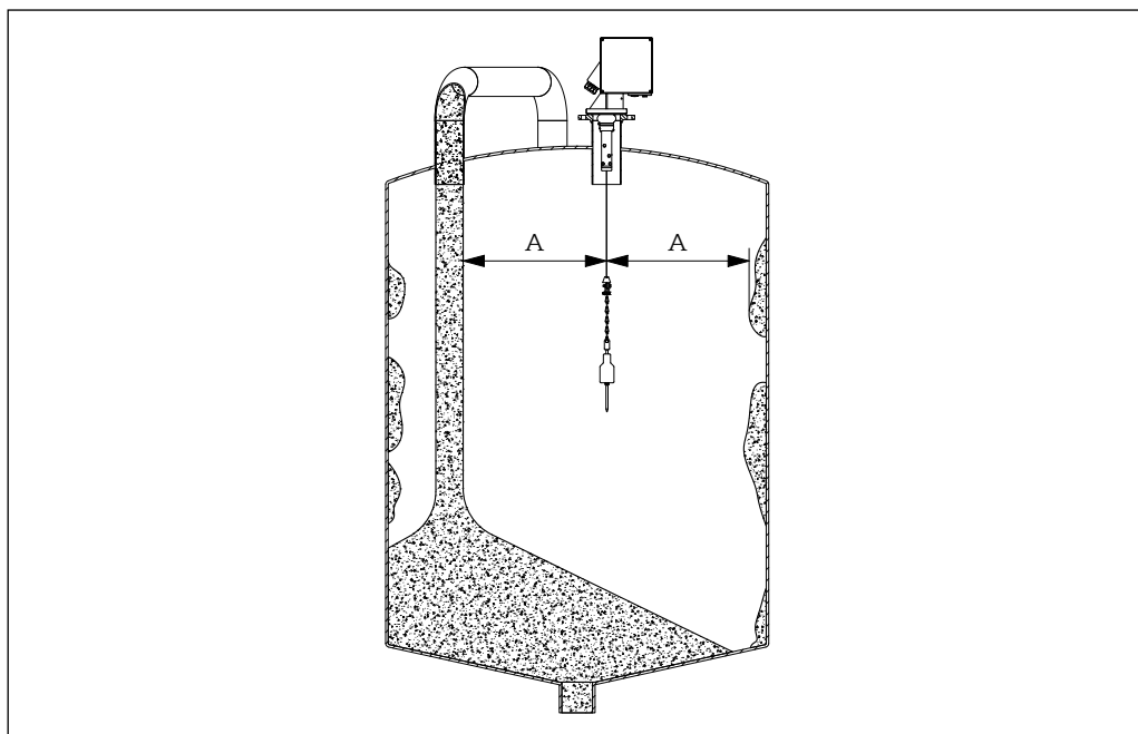
6 Installation position
