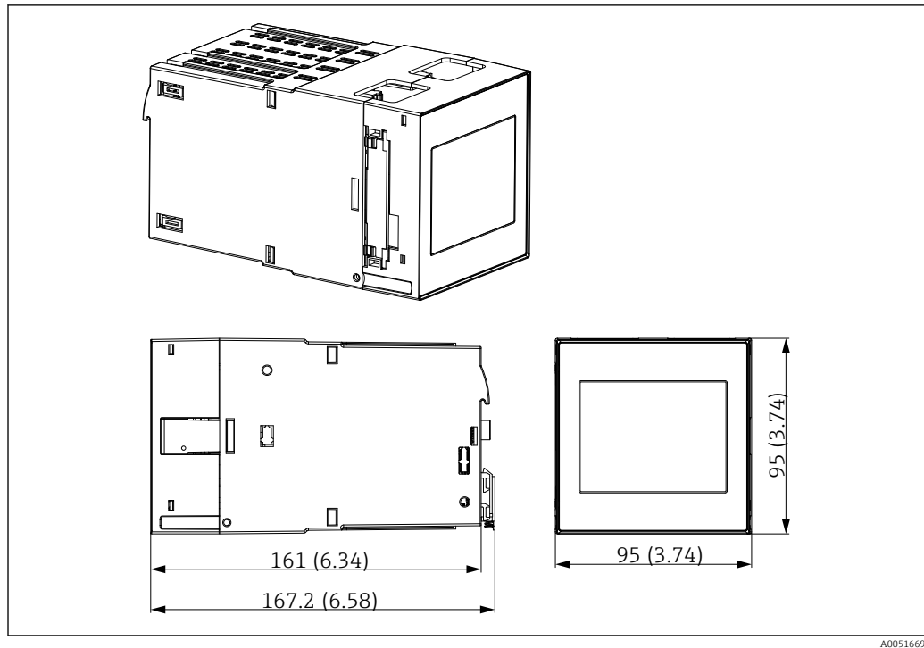
17 DIN rail housing. Unit of measurement mm (in)
