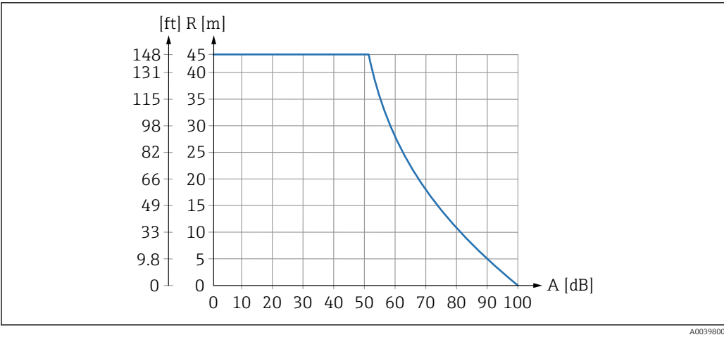
2 Range chart for ultrasonic sensors
