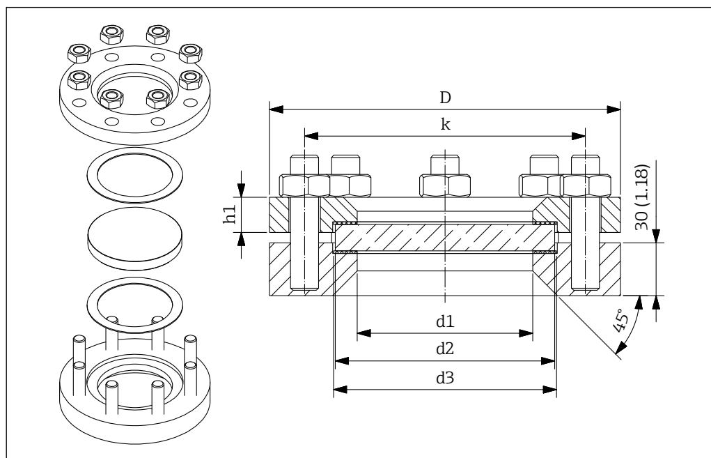
44 Dimensions sight glass fitting for processes up to 10 bar (145 psi). Unit of measurement mm (in)
