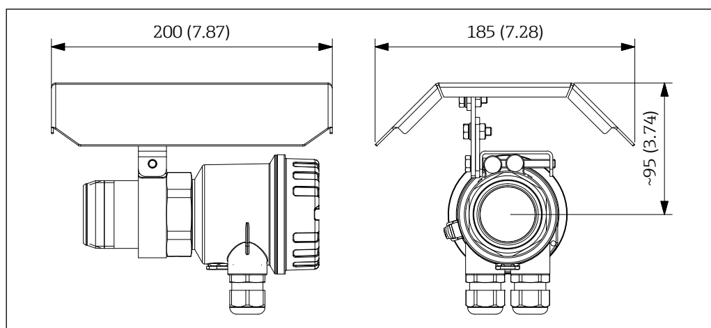
50 Dimensions weather protective cover. Unit of measurement mm (in)
