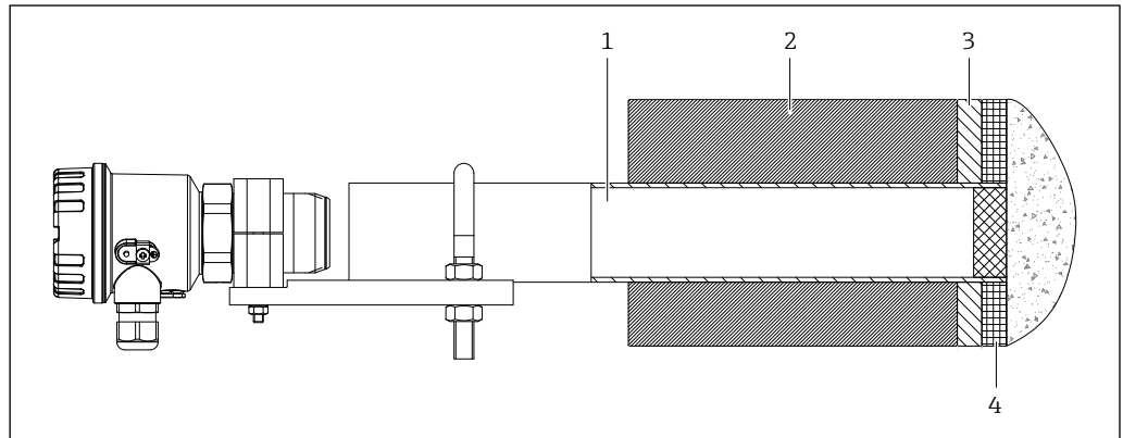
22 Mounting with spacer tube (wave guide)
