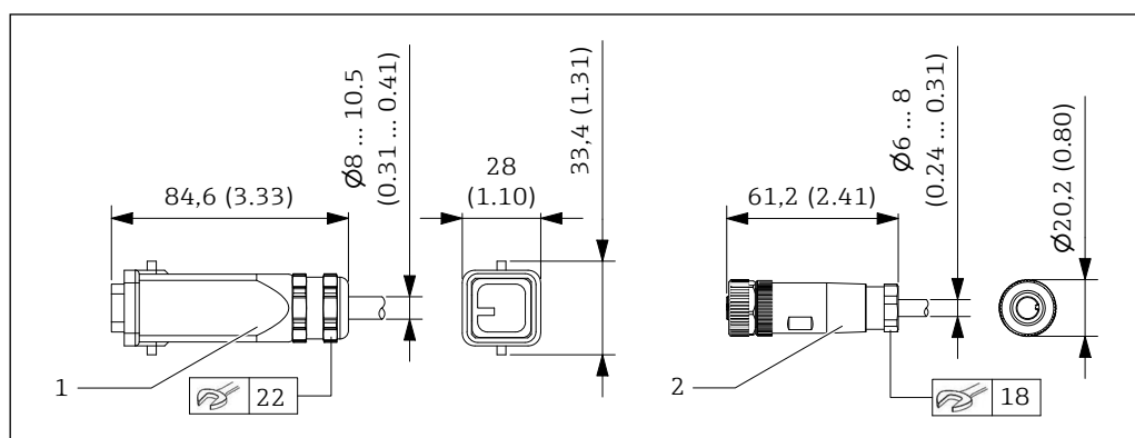
33 Mating connectors. Unit of measurement mm (in)
