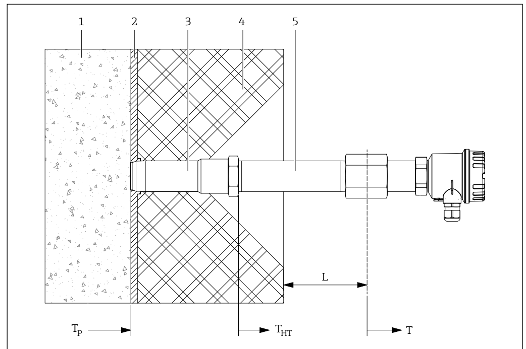
21 High temperature adapter with extension
