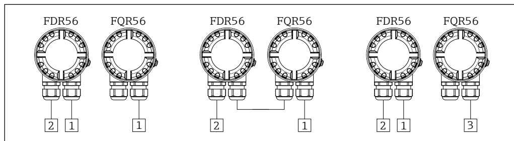
23 Connection examples
