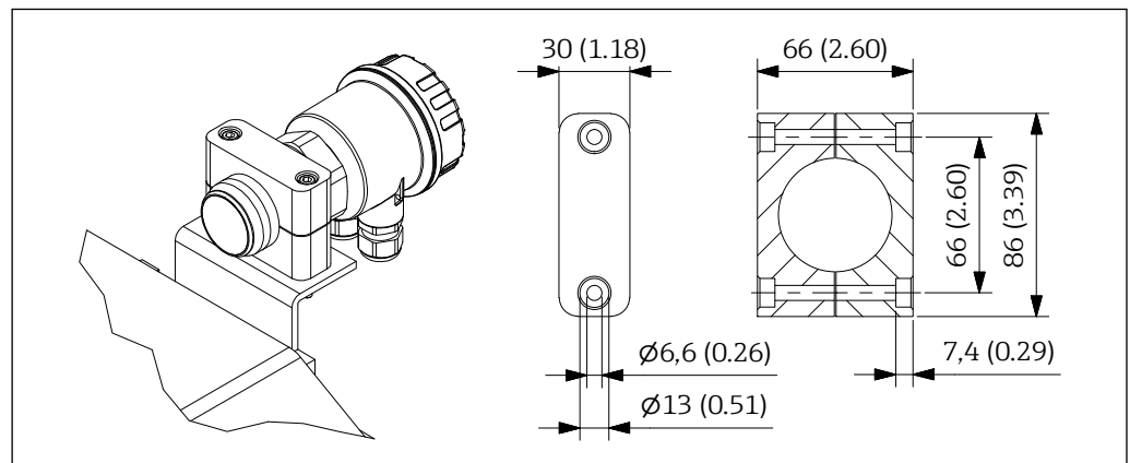
35 Dimensions mounting bracket. Unit of measurement mm (in)
