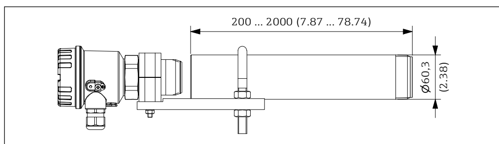
47 Dimensions spacer tube. Unit of measurement mm (in)
