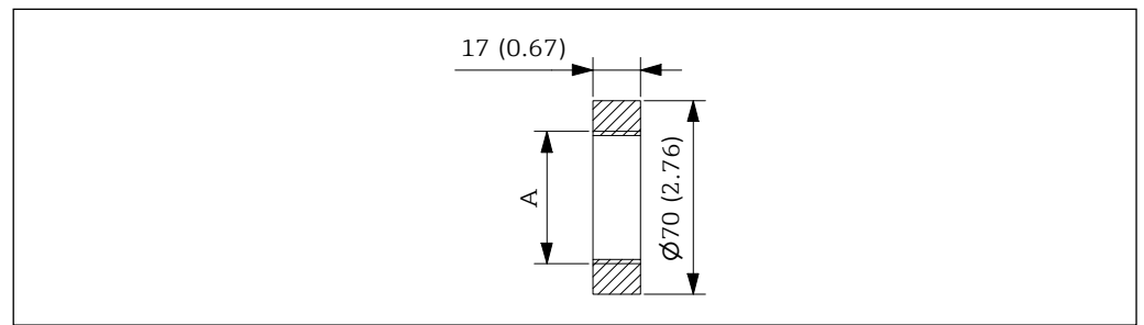
36 Dimensions FAR52-A. Unit of measurement mm (in)
