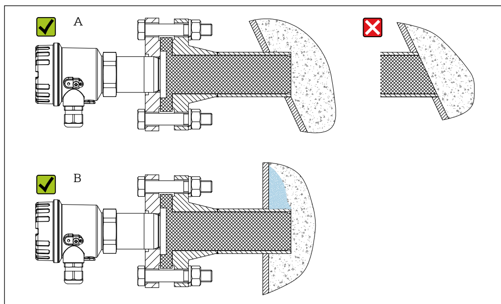
17 Mounting on process nozzle
