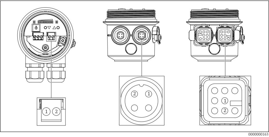
25 Supply circuit connection (Connector 1)
