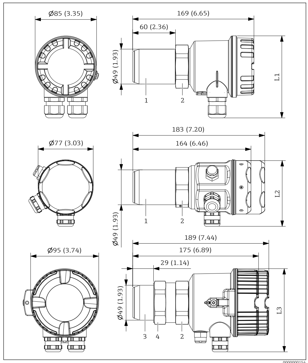
7 Mounting dimensions. Unit of measurement mm (in)
