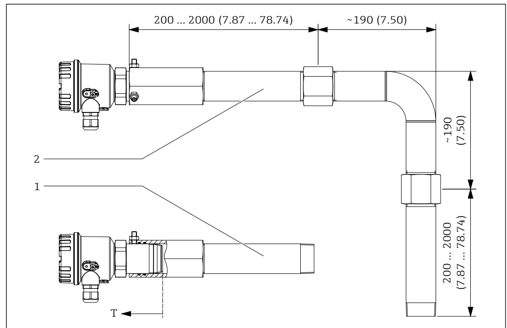
16 Wave guide FAR55. Unit of measure mm (in)
