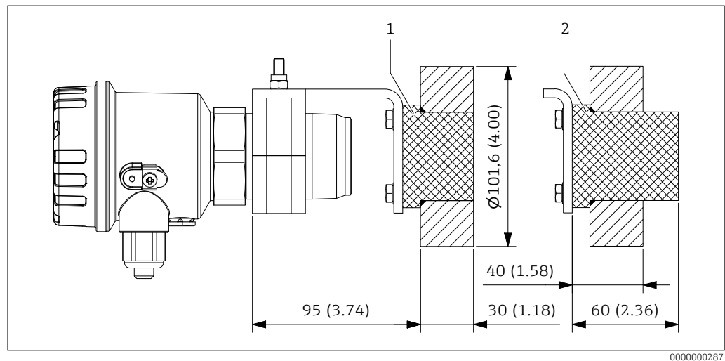
■ 38 Dimensions weld-in adapter. Unit of measurement mm (in)
