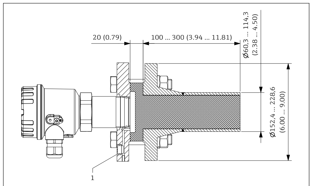
46 Dimensions weld-in nozzle. Unit of measurement mm (in)
