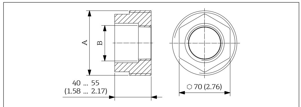
37 Dimensions FAR52-B. Unit of measurement mm (in)
