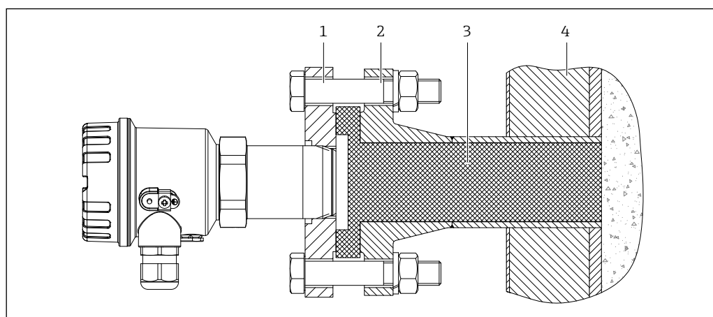
18 Weld-in nozzle FAR50
