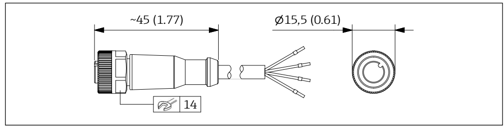
34 Connection cable with M12 plug. Unit of measurement mm (in)
