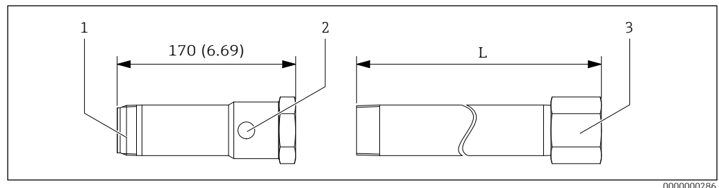
49 Dimensions high temperature adapter with extension. Unit of measurement mm (in)
