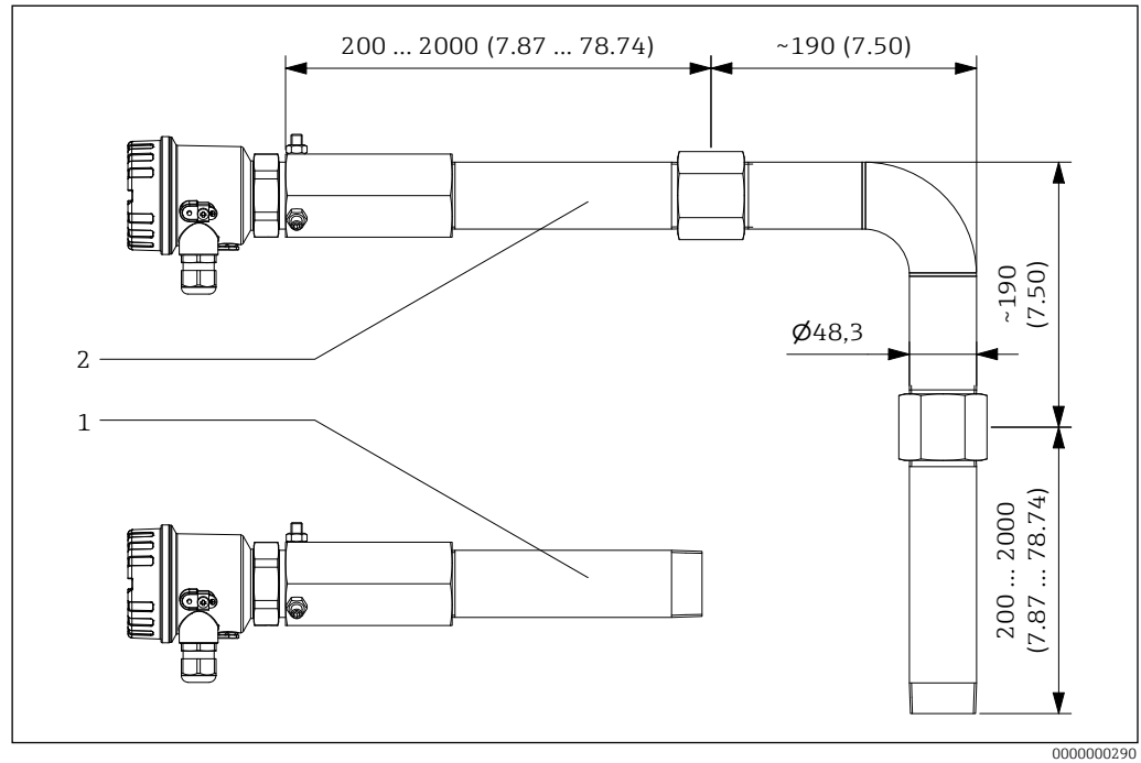
48 Dimensions wave guide. Unit of measurement mm (in)
