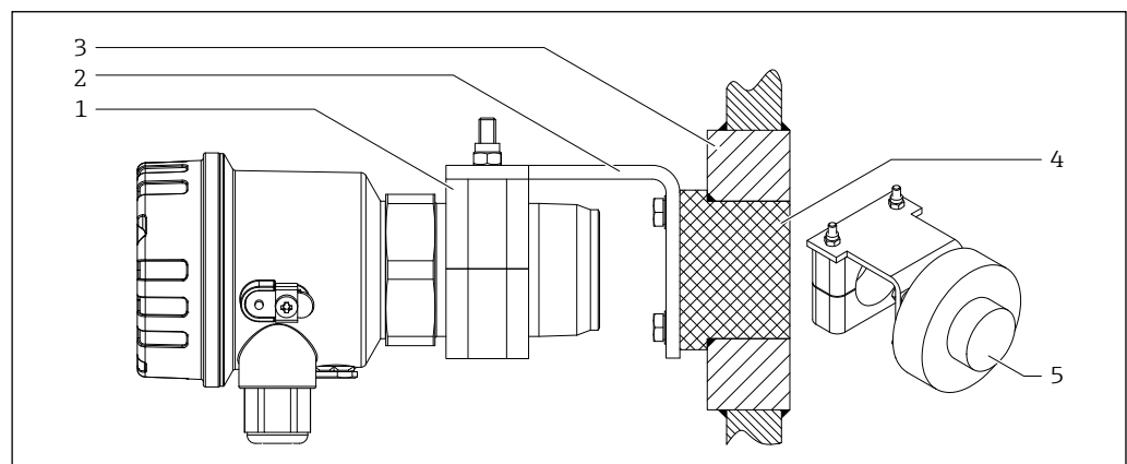
13 Weld-in adapter with mounting arm. Unit of measurement mm (in)
