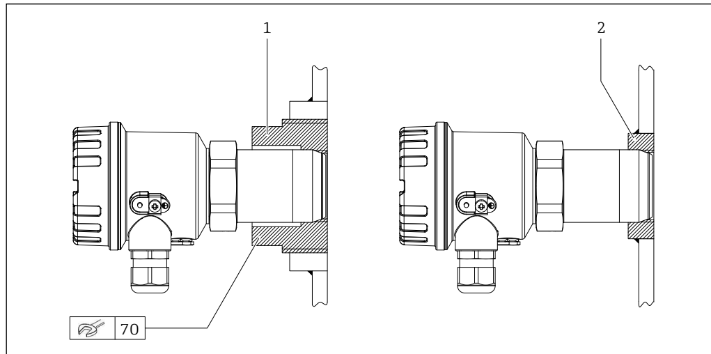
10 Weld-in or screw-in adapter FAR52. Unit of measurement mm (in)
