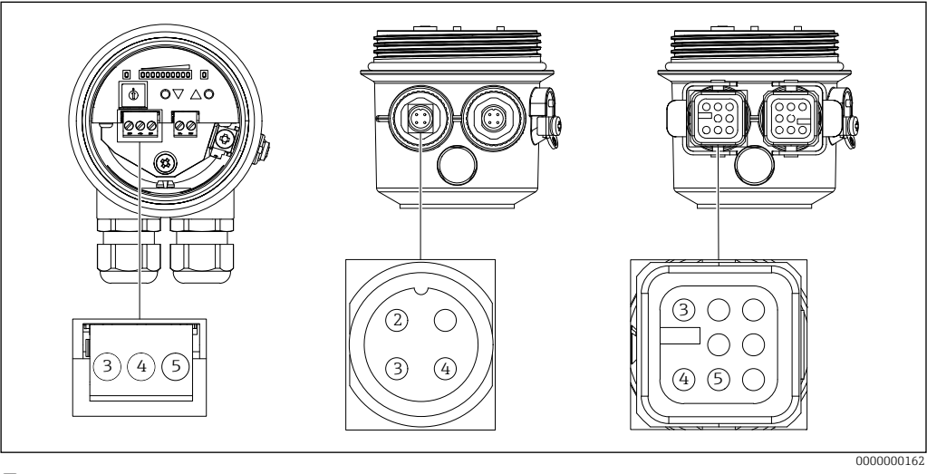
26 Connection signal circuit (Connector 2)
