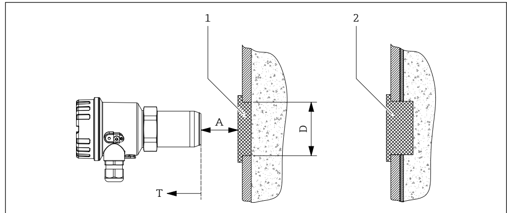
12 Mounting in front of microwave-impermeable process wall
