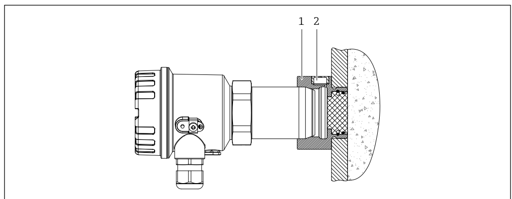
20 High pressure adapter
