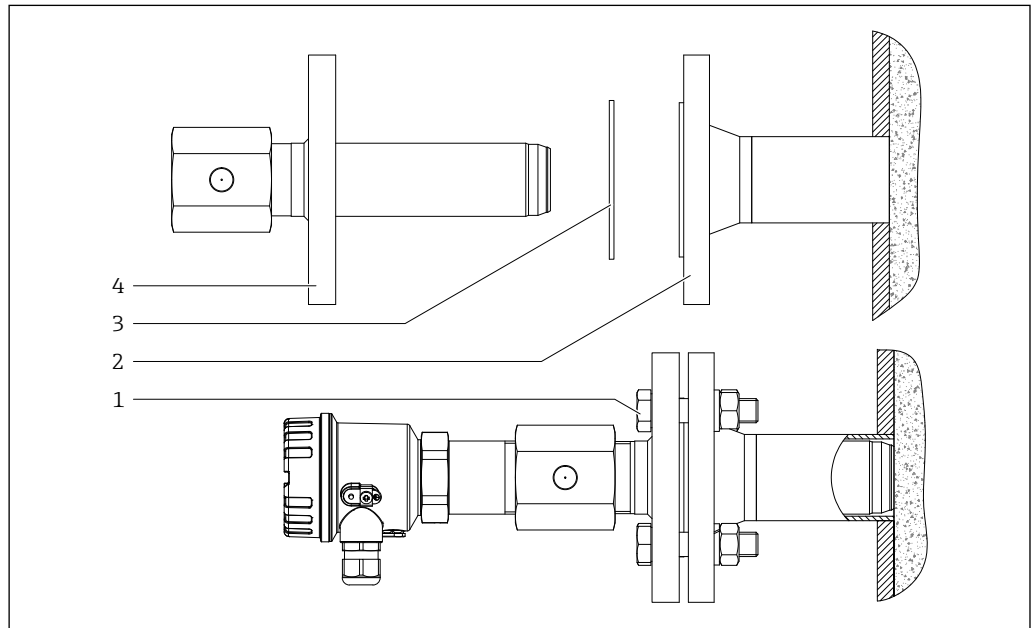
19 Insertion adapter FAR51
