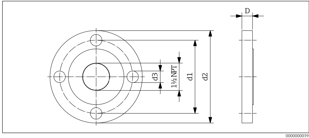
40 Dimensions mounting flange (Connection dimensions according to ANSI/ASME B16.5)
