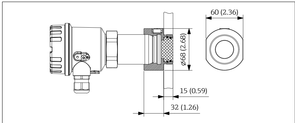
41 Dimensions high pressure adapter. Unit of measurement mm (in)
