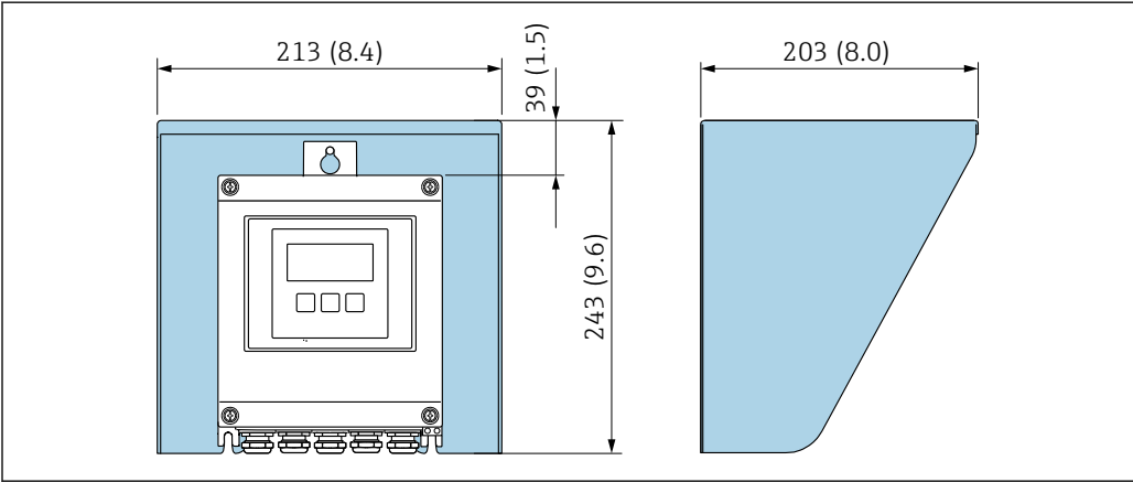
40 Weather protection cover for Proline 500 – digital; unit mm (in)
