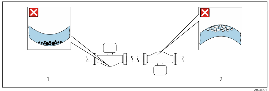
15 Orientation of sensor with curved measuring tube
