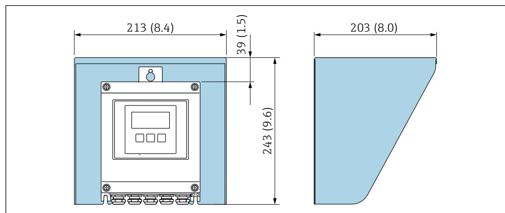
20 Weather protection cover for Proline 500 – digital; unit mm (in)
