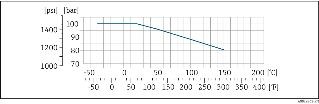
31 With connection material 1.4404 (316/316L)
