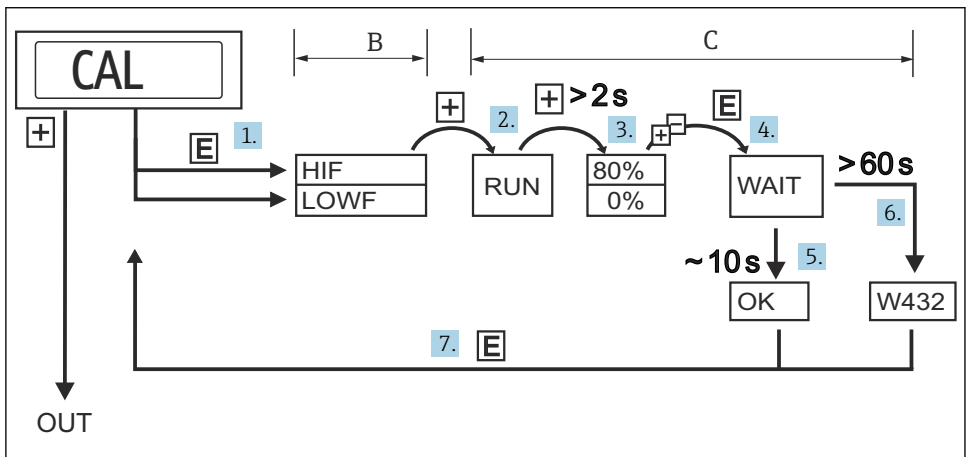
9 Navigating the 'Learn' function taking the example of the Calibration (CAL) function group
