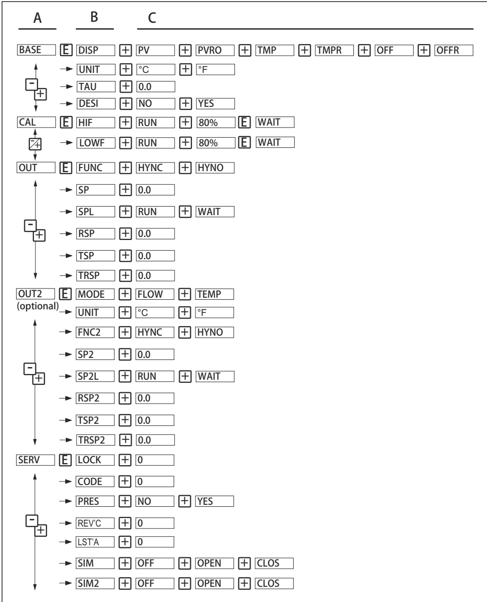
11 Operating menu
