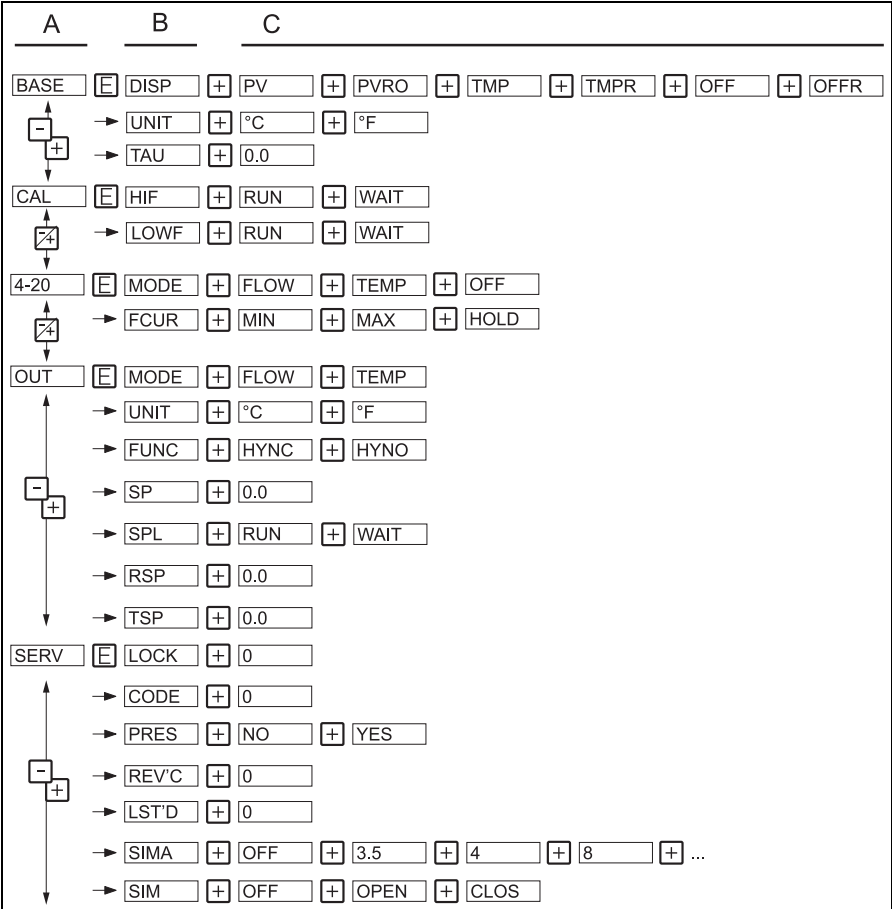
Fig. 16: Operating menu: A function groups, B functions, C settings
