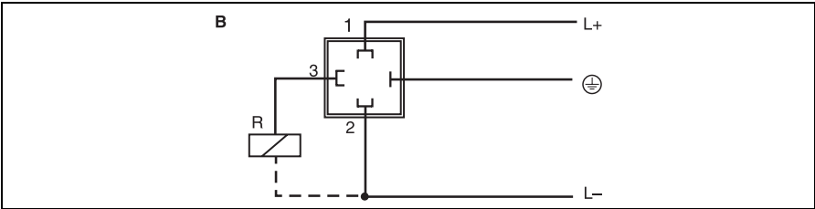
Fig. 10: Flowphant® T with M16x1.5 valve connector or NPT ½"
