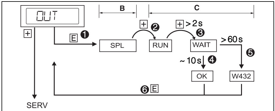
Fig. 14: Navigating the 'Learn' switch point
