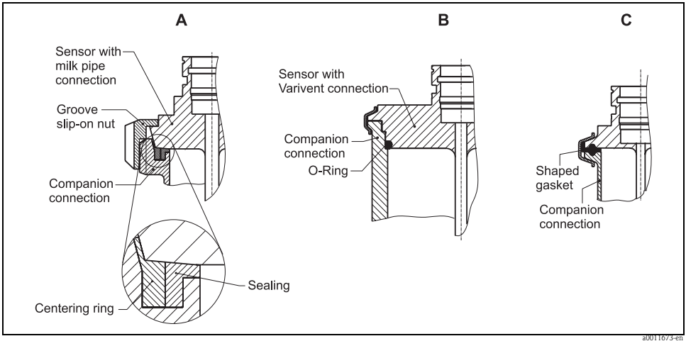
Fig. 8: Installation in hygienic processes
