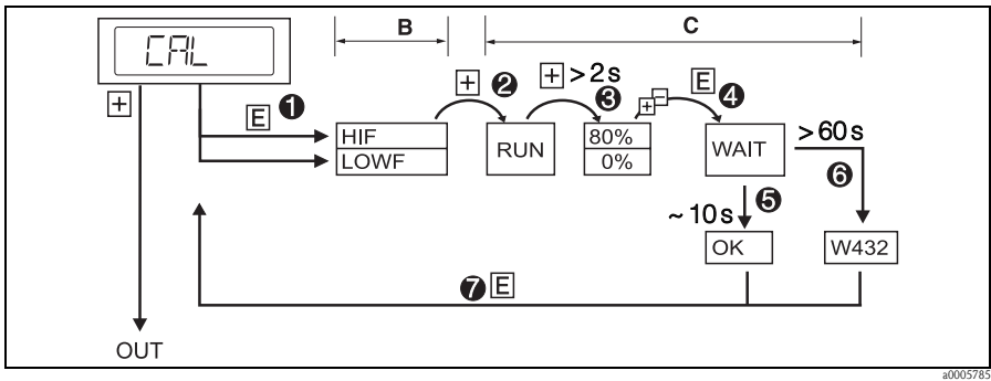
Fig. 13: Navigating the 'Learn' function using the Calibration (CAL) function group as an example
