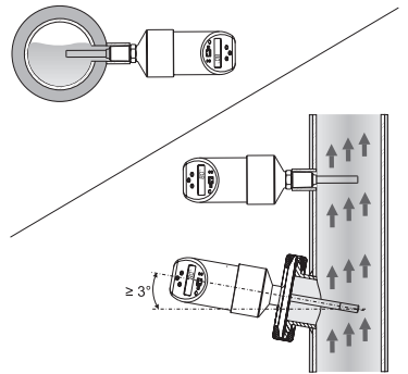
Fig. 6: Correct orientation
