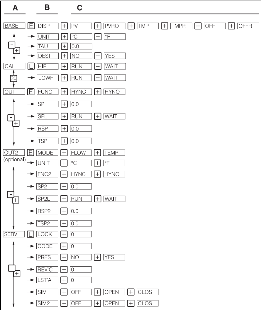
Fig. 15: Operating menu: A function groups, B functions, C settings
