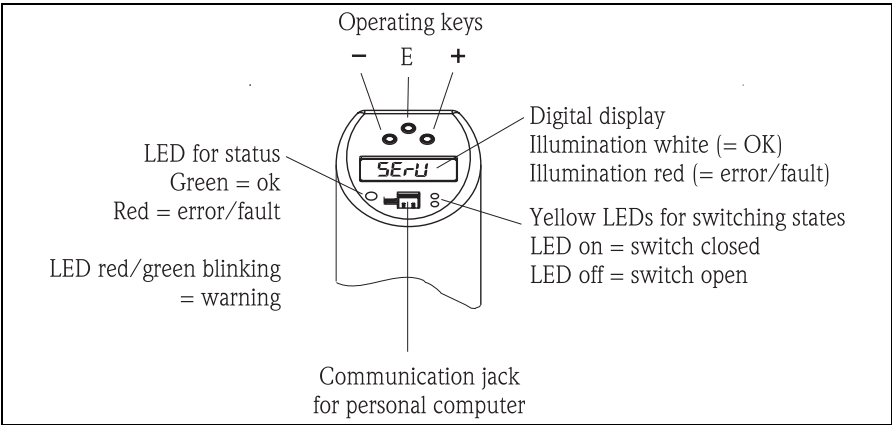
Fig. 11: Position of operating elements and possibilities for display
