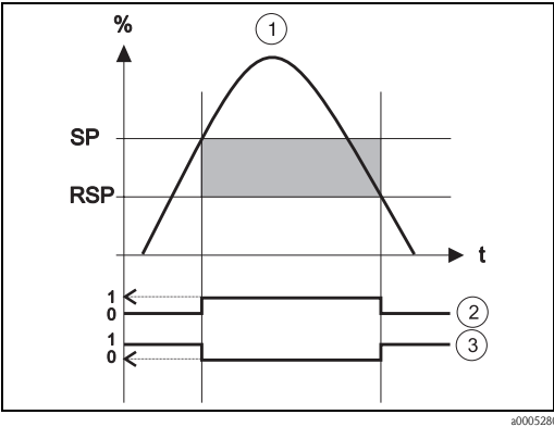
Fig. 17: ① Hysteresis function, ② NO contact, ③ NC contact
