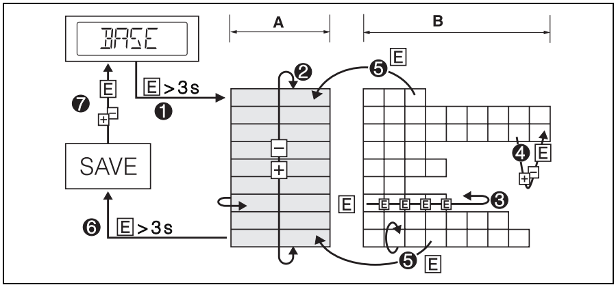
Fig. 12: Navigating in the operating menu
