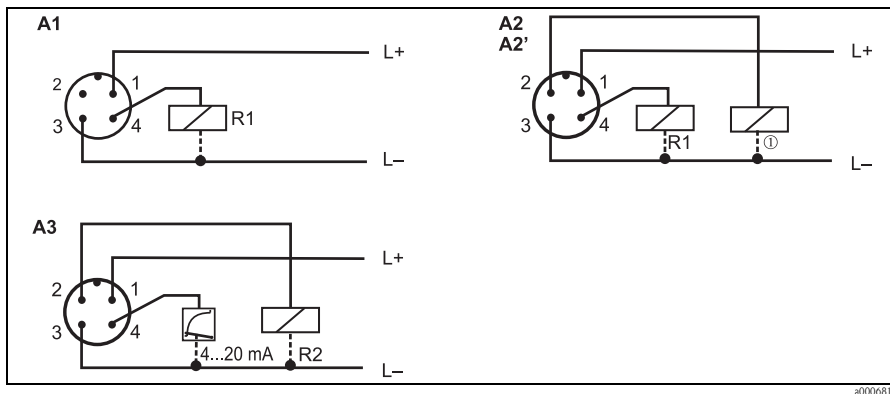
Fig. 9: Flowphant® T with M12x1 connector
