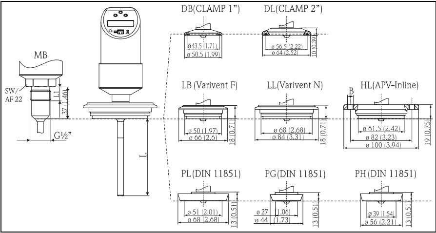
Fig. 4: Hygienic process connections. All dimensions in mm (inch)
