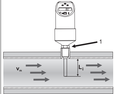
Fig. 5: Installation conditions
