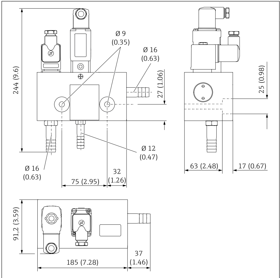
4 Dimensions in mm (in)
