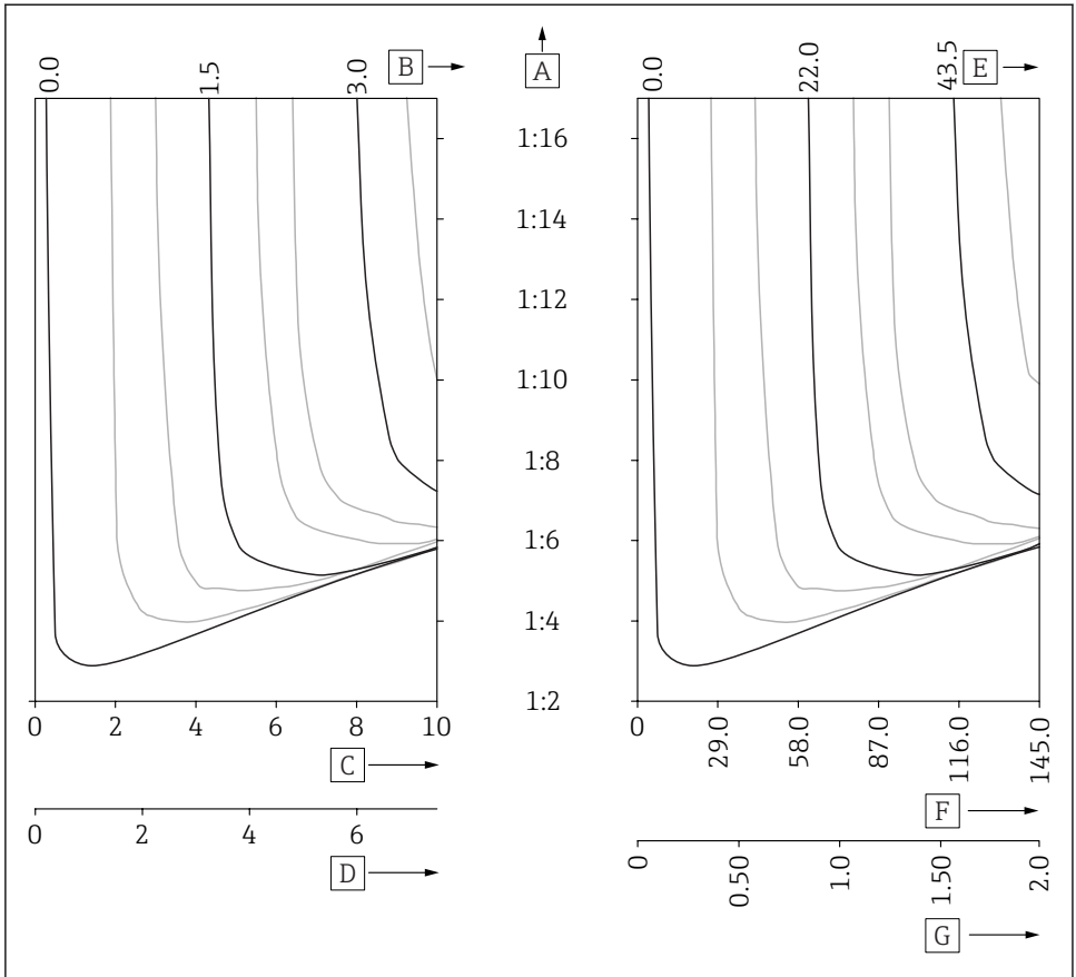
10 Characteristic curve when metering valve is completely open
