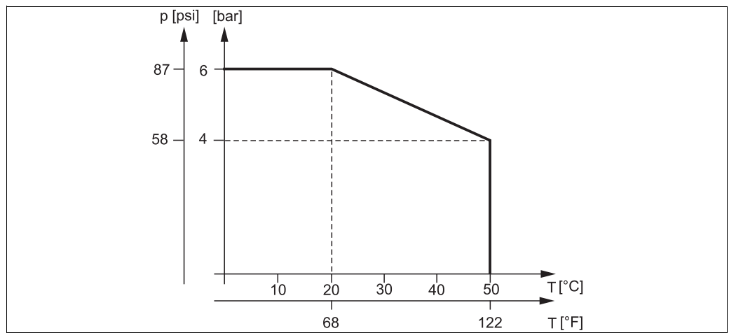
Pressure-temperature diagram
