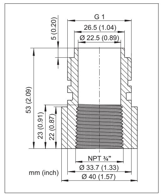
Adapter G 1 to NPT ¾
