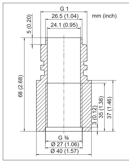
Adapter G 1 to G ¾
