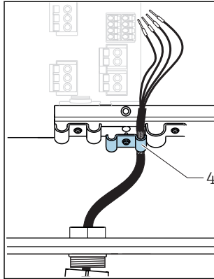
9 Insert the cable
