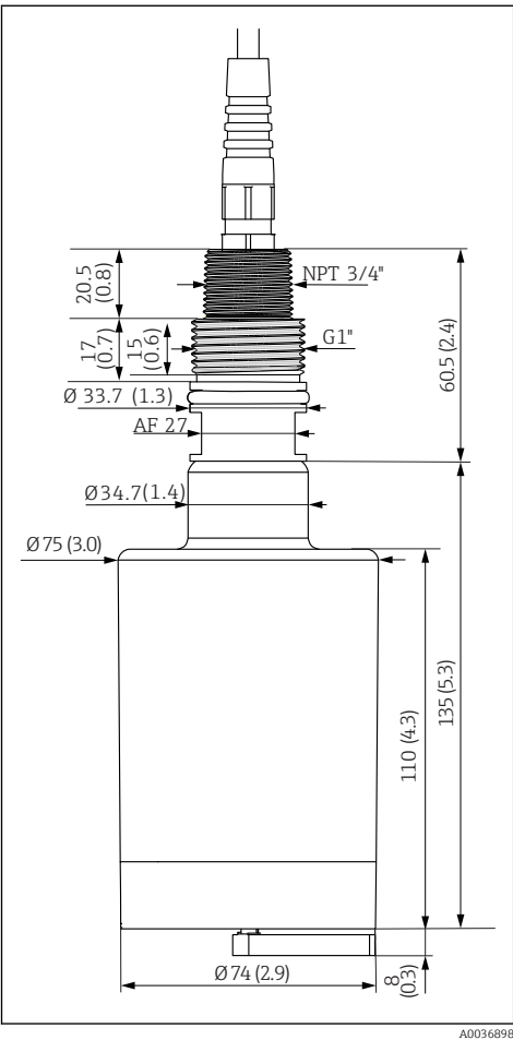
3 Dimensions for sensor with wiper. Dimensions: mm (in)
