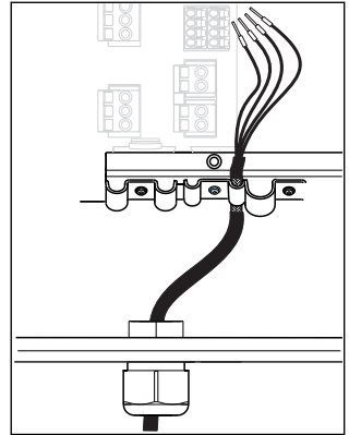
10 Tighten screw (2 Nm)
