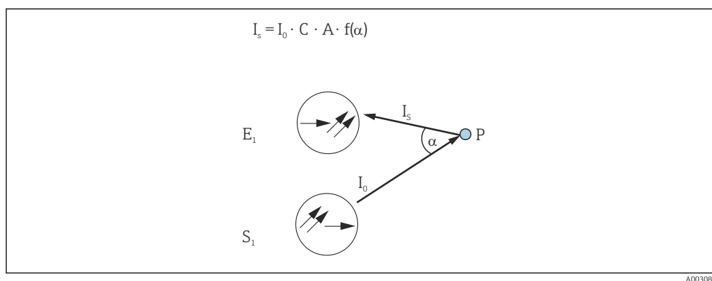
7 Principle of backscattered light method
