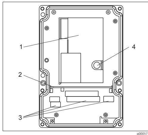
View into the field instrument
