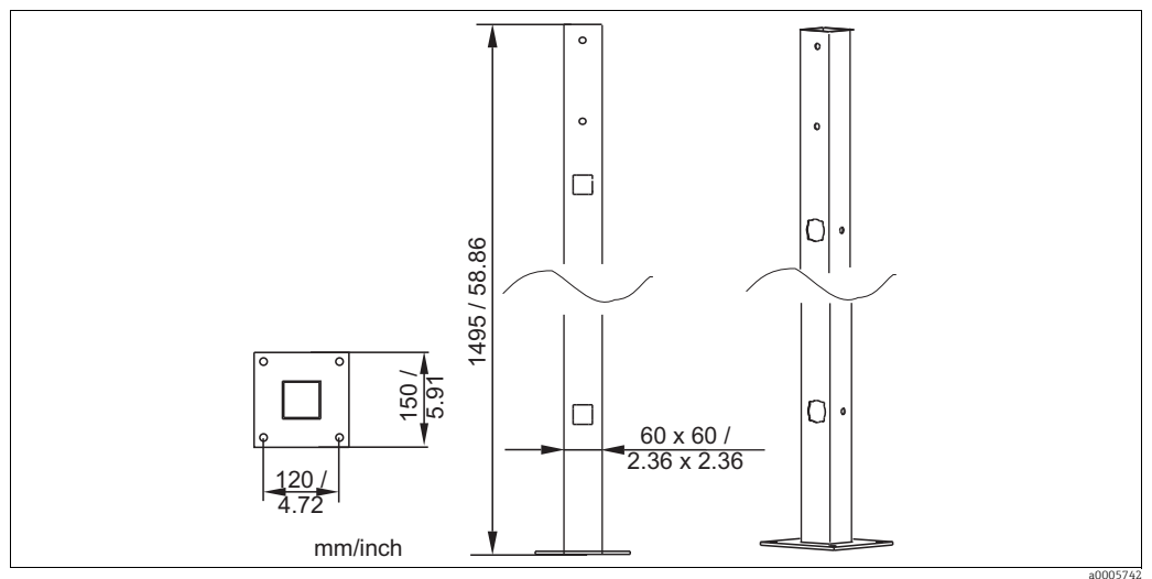
Universal post
