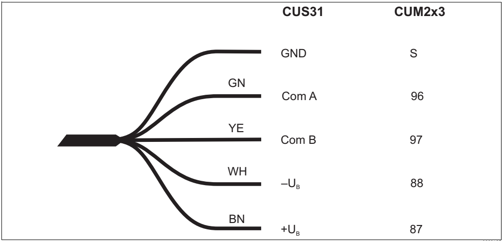
Measuring cable (fixed cable) resp. extension cable (CYK81)
