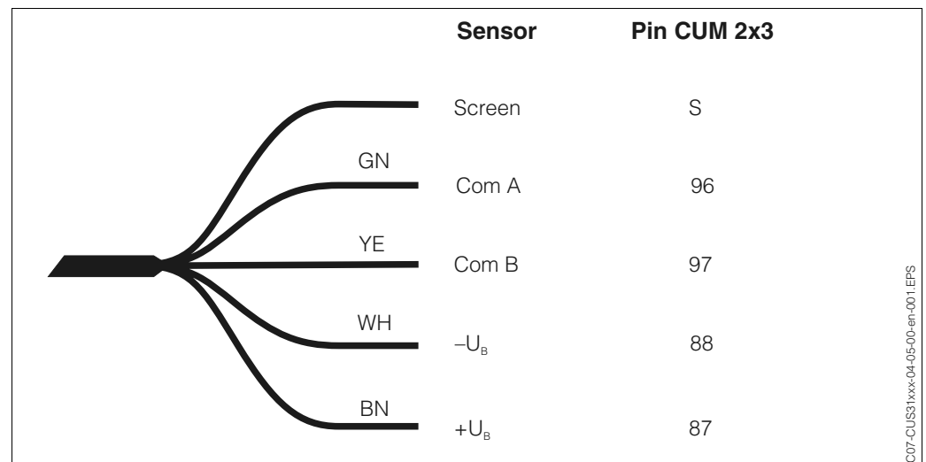
Fig. 13: Measuring cable CYK 8 (fixed cable) or CYK 81 (extension cable)
