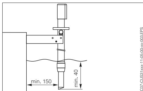
Fig. 5: Minimum distance when installing in -CYA 611 with pendulum frame
