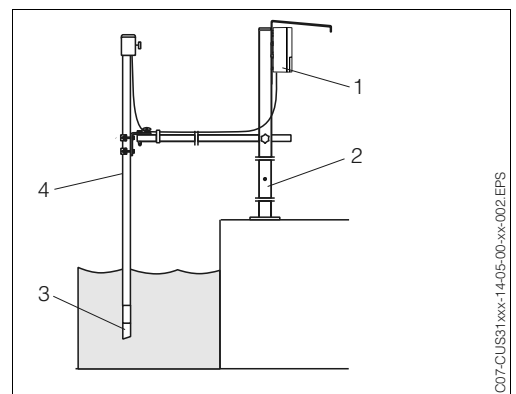
Fig. 2: Measuring system with immersion assembly
