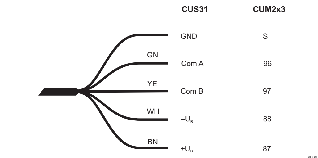
Fig. 13: Measuring cable (fixed cable) resp. extension cable (CYK81)
