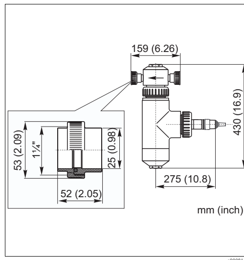
Fig. 4: CUS31-**S (with assembly S)
