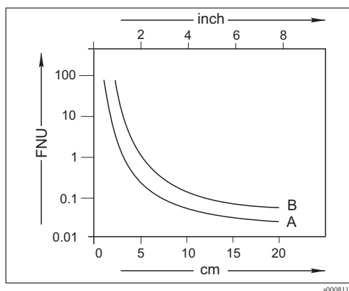
Fig. 5: Effect of the distance from the wall or bottom
