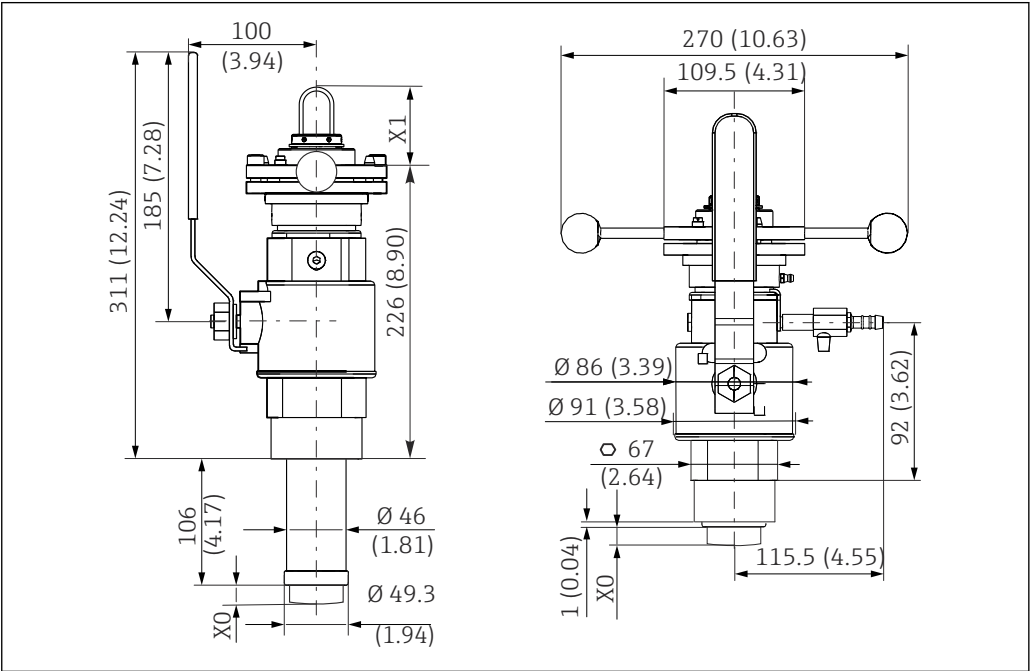
7 Dimensions in mm (in) X0, Dimensions depend on the sensor X1, X2
