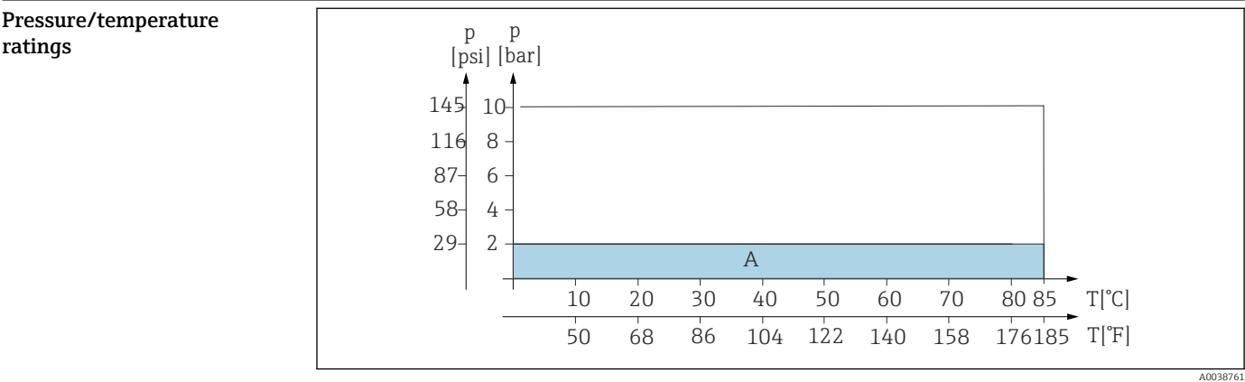
6 Pressure/temperature ratings A Range in which the assembly can be operated manually
