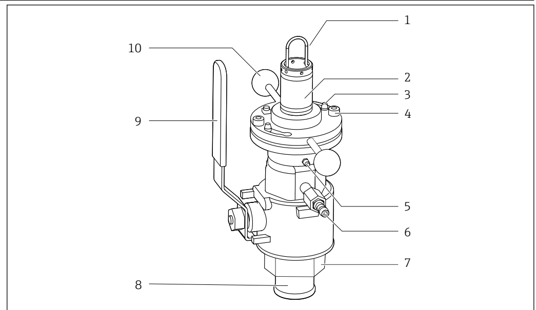
1 Assembly in operational state (ball valve open)
