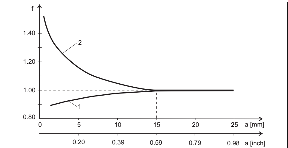
Fig. 7: Relation between the installation factor f and the wall distance
