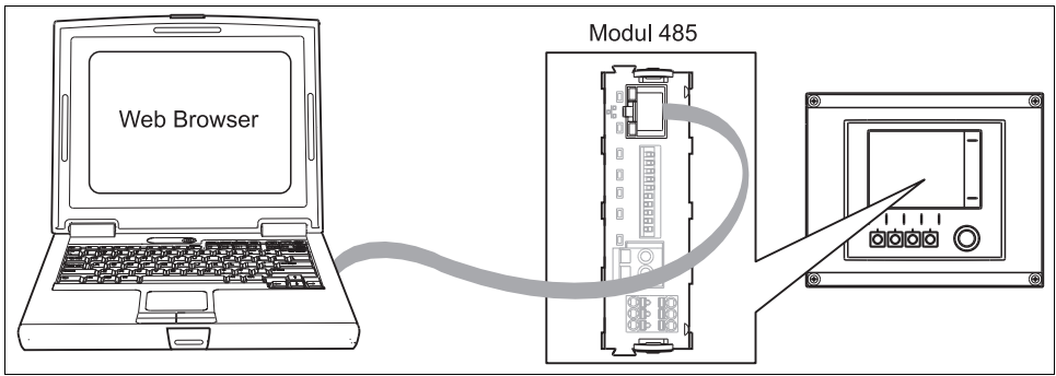
Fig. 11: Ethernet connection
