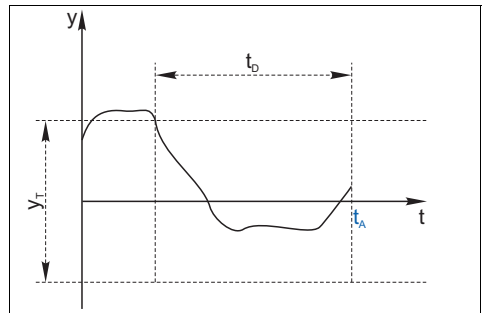
Fig. 9: Stagnating signal, alarm is triggered
