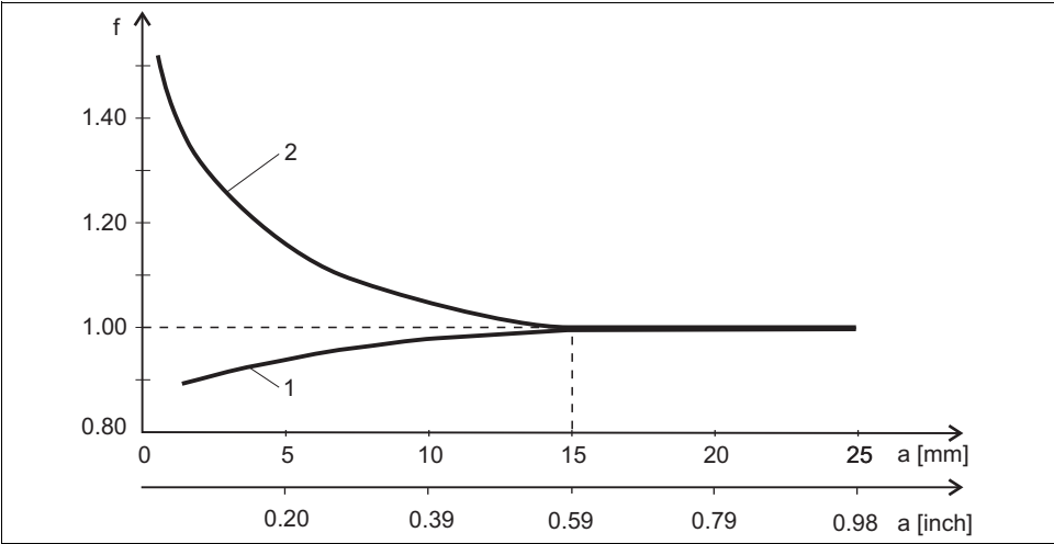
Fig. 10: Relation between the installation factor f and the wall distance
