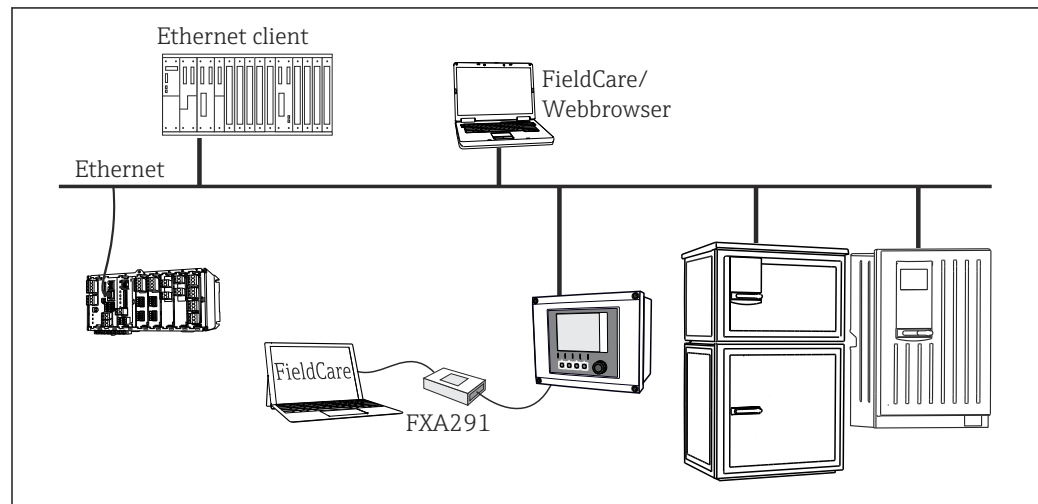
12 Example of system integration via web server
