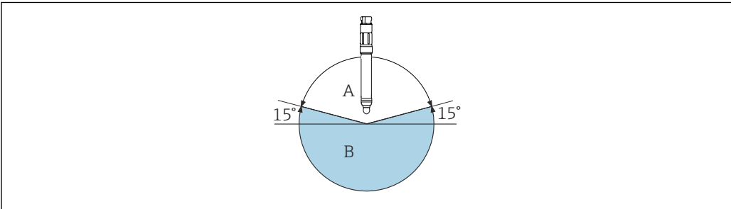
4 Installation angle at least 15^\circ from the horizontal
