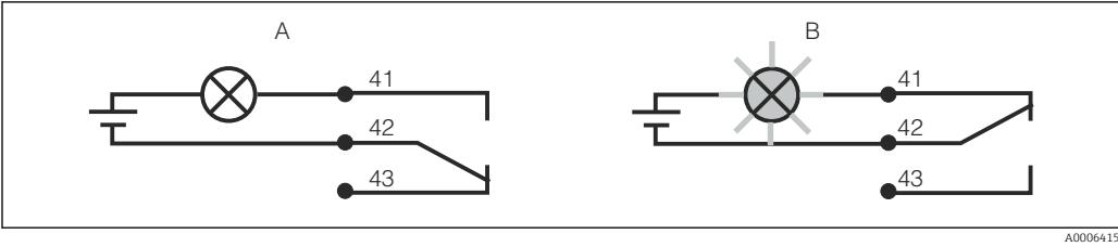
25 Recommended fail-safe switching for the alarm contact
