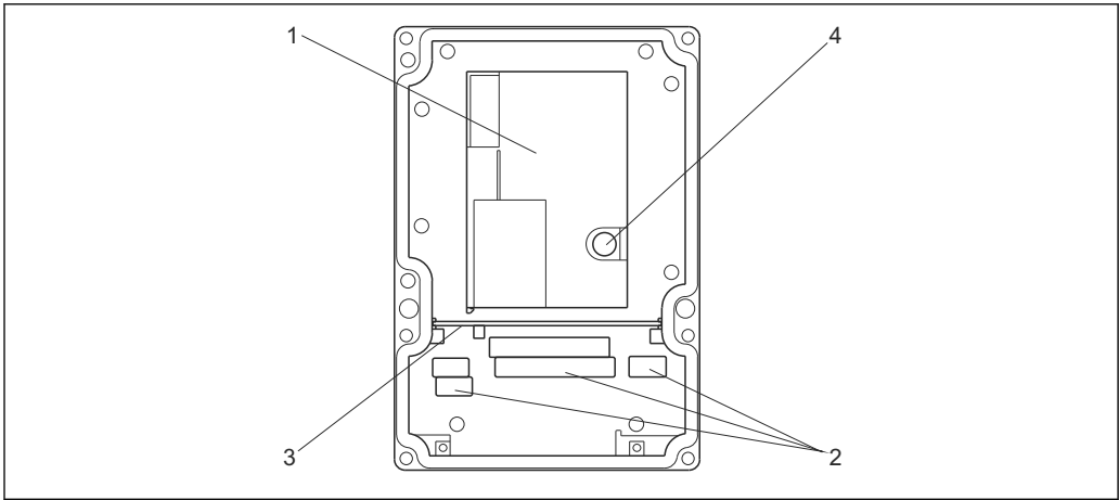
3 View into the field housing 1 Removable electronics box 2 Terminals 3 Partition plate 4 Fuse
