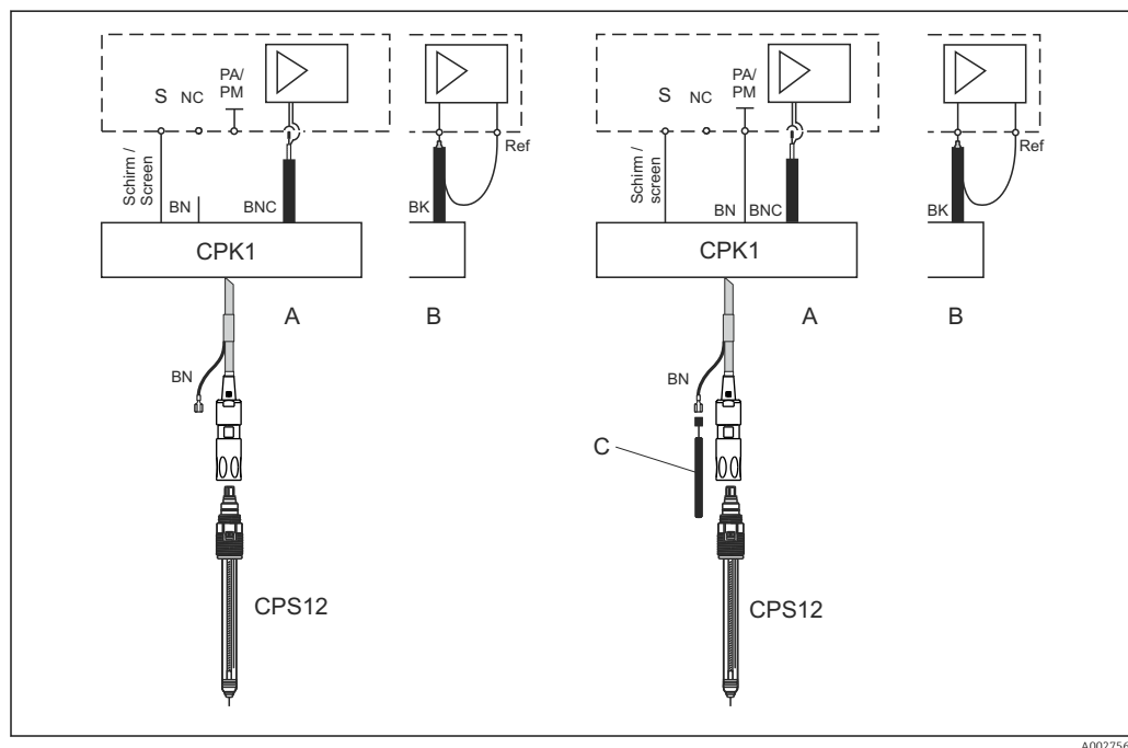
18 Asymmetrical (without PML) and symmetrical (with PML) connection of ORP electrodes
