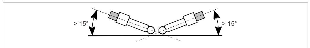
46 Permitted angle of installation for glass electrodes
