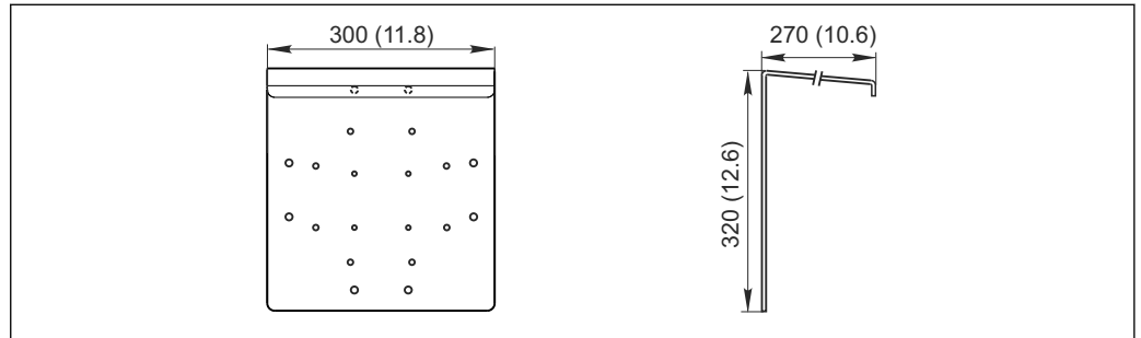
49 Dimensions in mm (inch)
