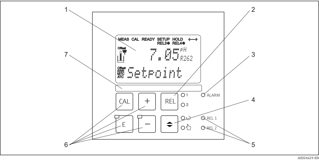
27 Operating elements
