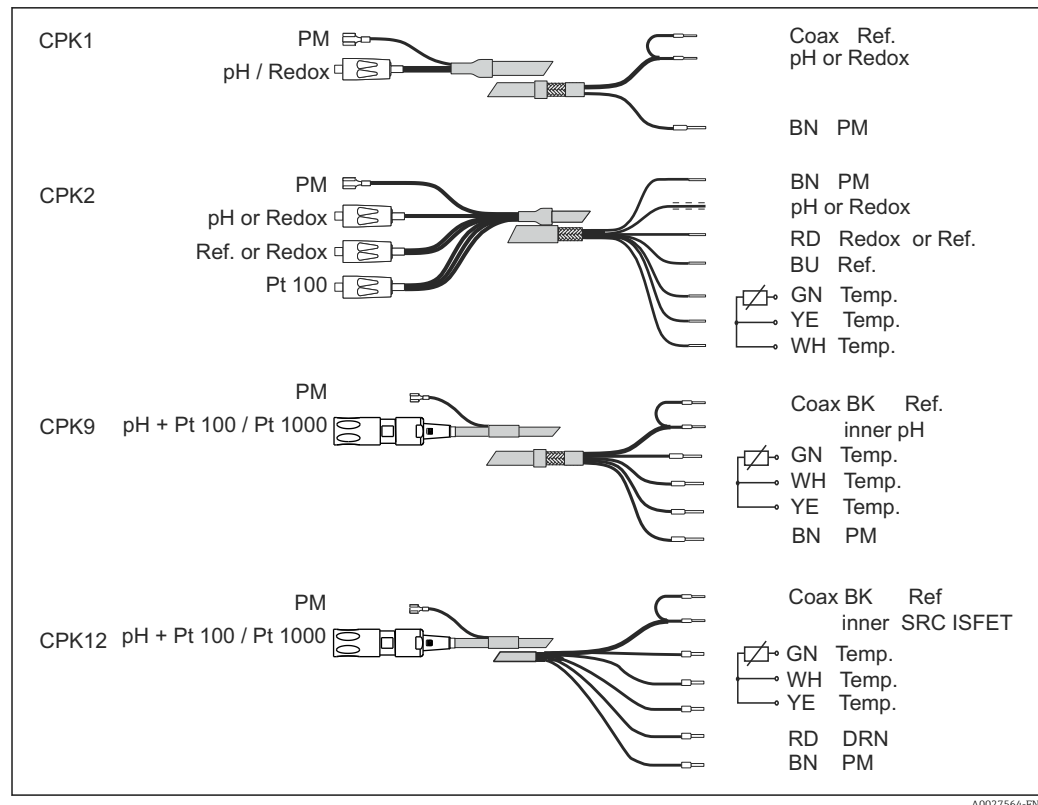
12 Structure of the special measuring cables
