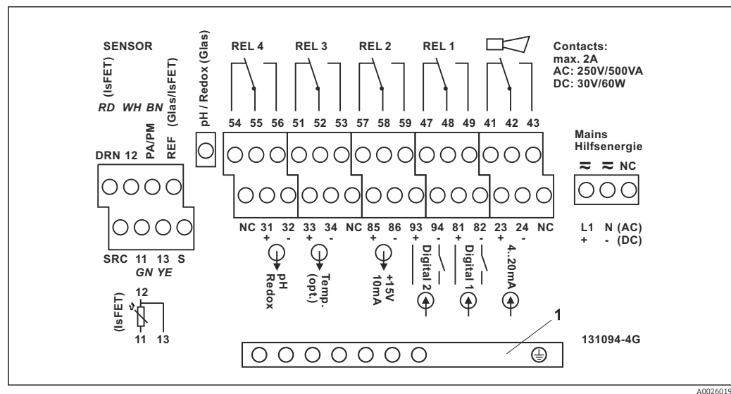
10 Field device connection compartment sticker
