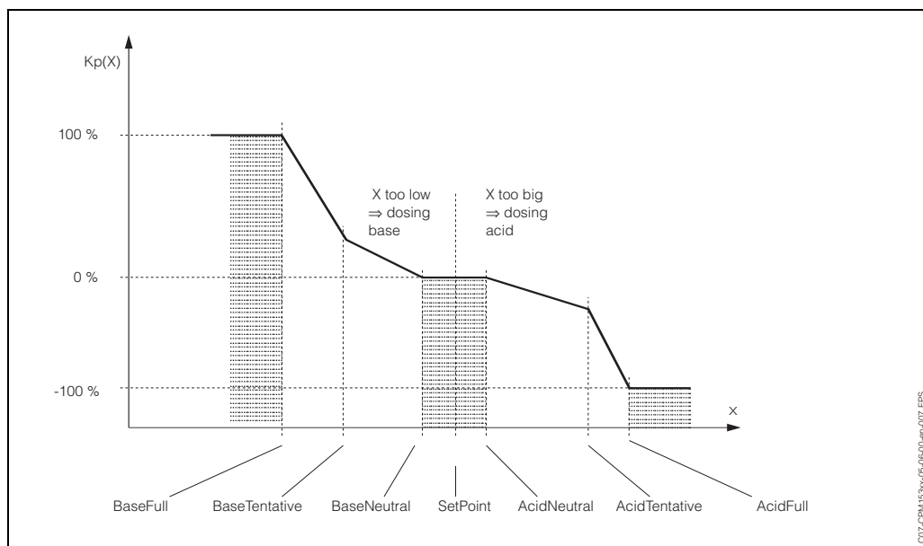
Fig. 22: Diagram to describe the most important corner points for control
