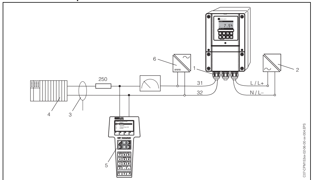
Fig. 5: Electrical connection of the HART® handheld terminal DXR 275
