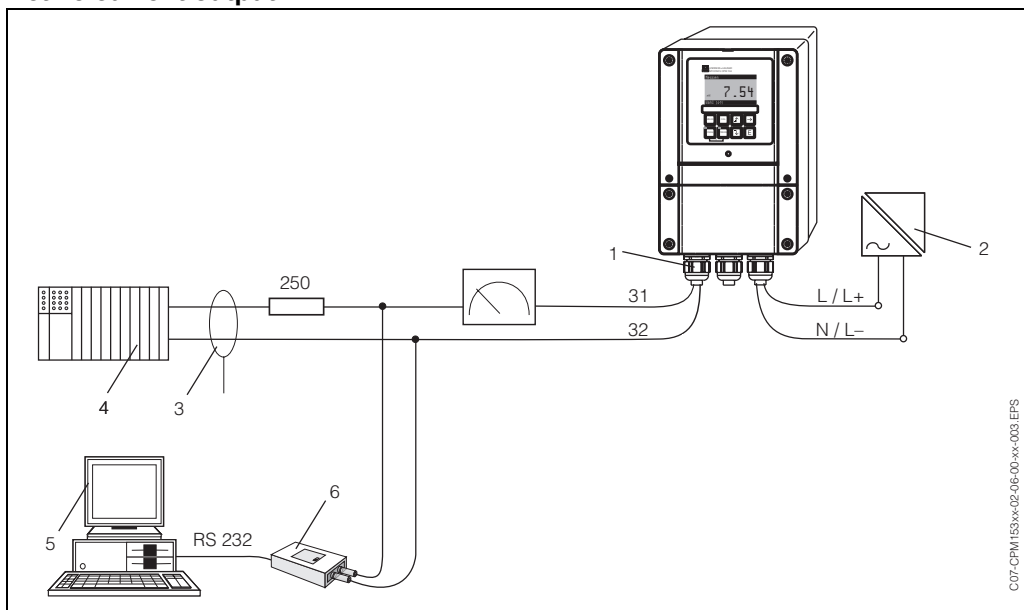
Fig. 6: Electrical connection of the Commubox FXA 191
