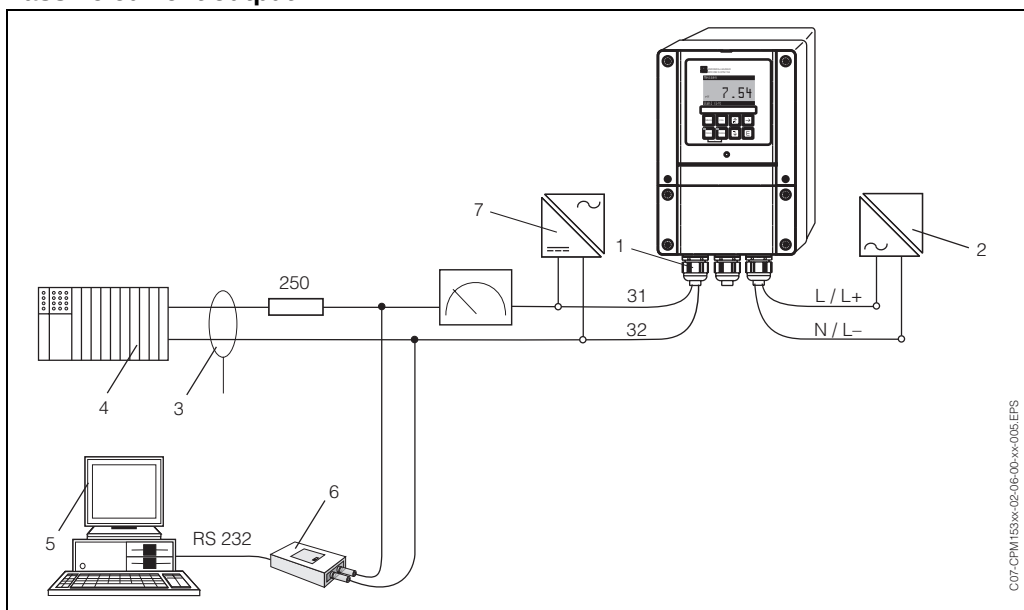
Fig. 7: Electrical connection of the Commubox FXA 191
