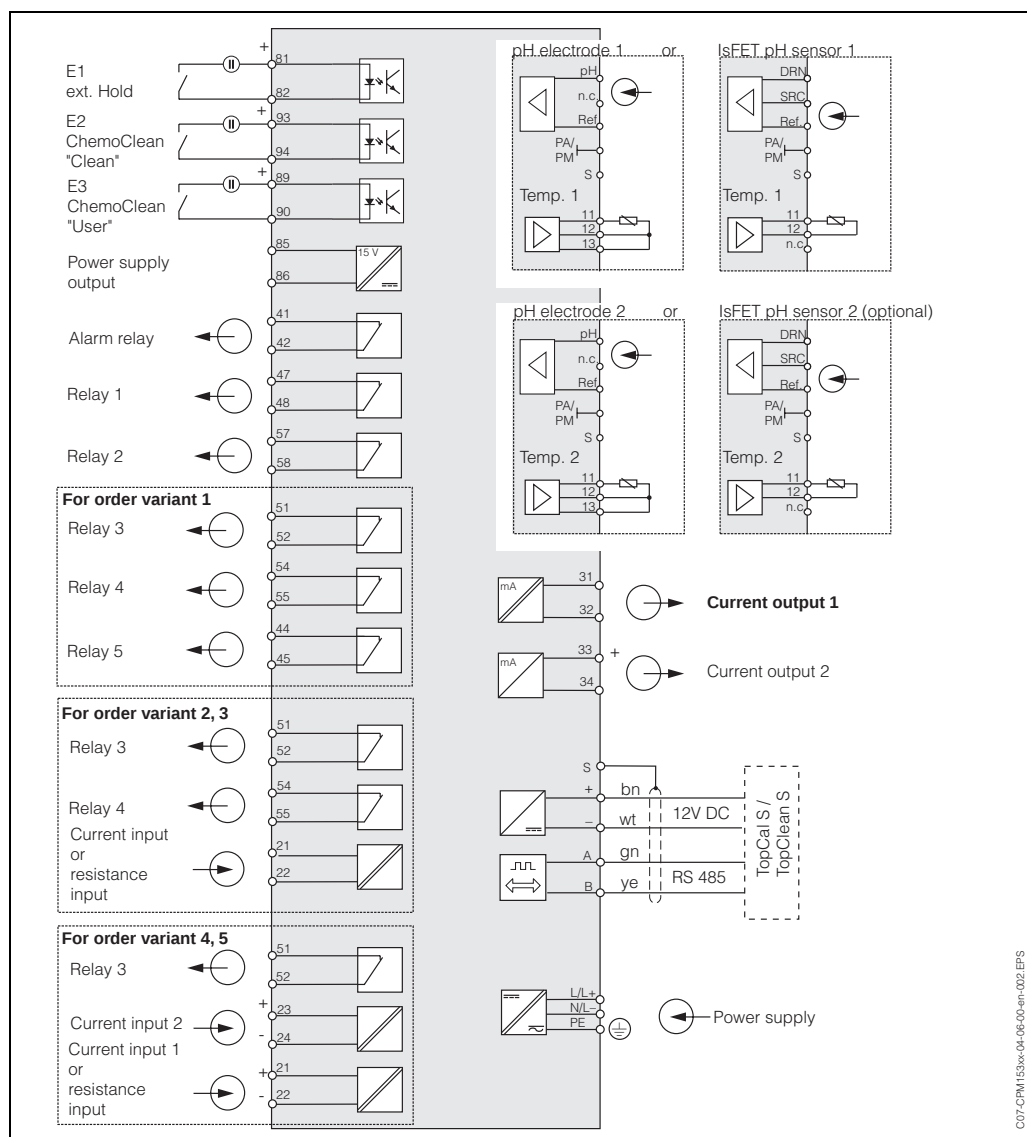
Fig. 3: Electrical connection of Mycom S CXM 153 HART®
