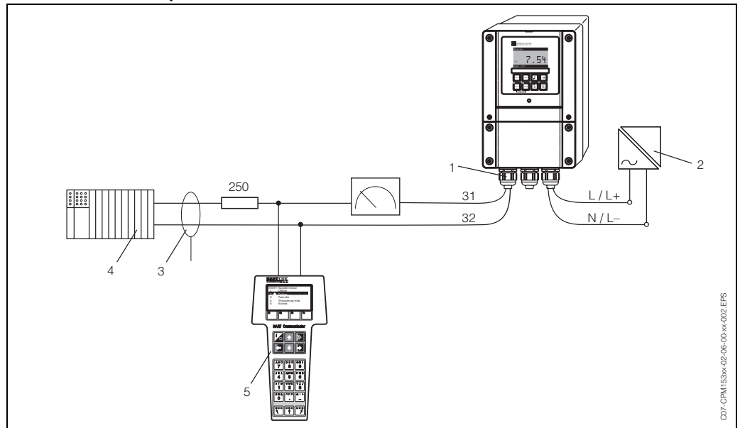
Fig. 4: Electrical connection of the HART® handheld terminal DXR 275
