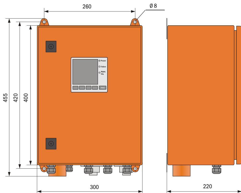
Figure 31 MCU-P control unit
