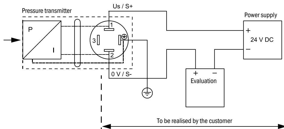
Pressure sensor connection
