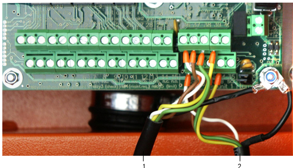
Figure 7 Connections of sender/receiver units
