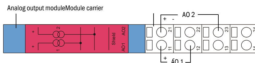
Terminal assignment analog output module
