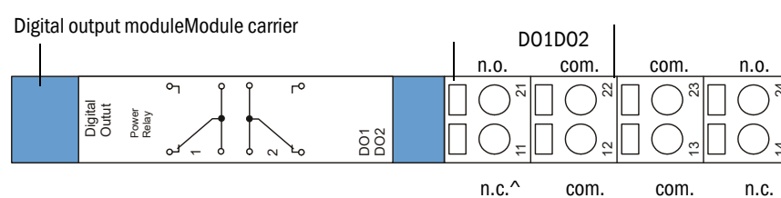
Terminal assignment digital output module Power Relay
