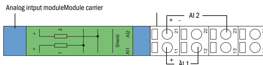
Terminal assignment analog input module
