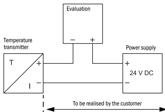
Temperature sensor connection
