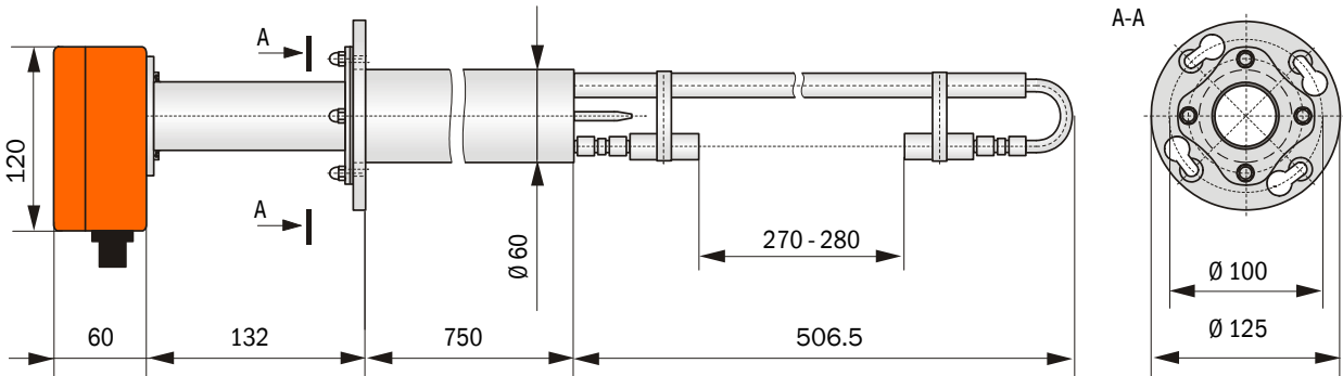
Figure 26 FLSE100-PR sender/receiver unit
