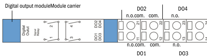
Terminal assignment digital output module Signal Relay (4 make contact elements)
