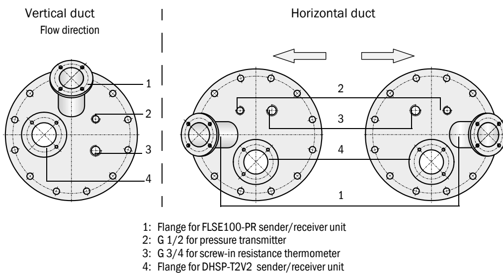
Combo flange alignment
