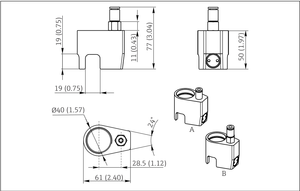
15 Dimensions in mm (inch) A Compressed air cleaning COS61/61D OD 6/8 mm (additional information → 31) B Compressed air cleaning COS61/61D OD 6.35 mm (¼") (additional information → 31)
