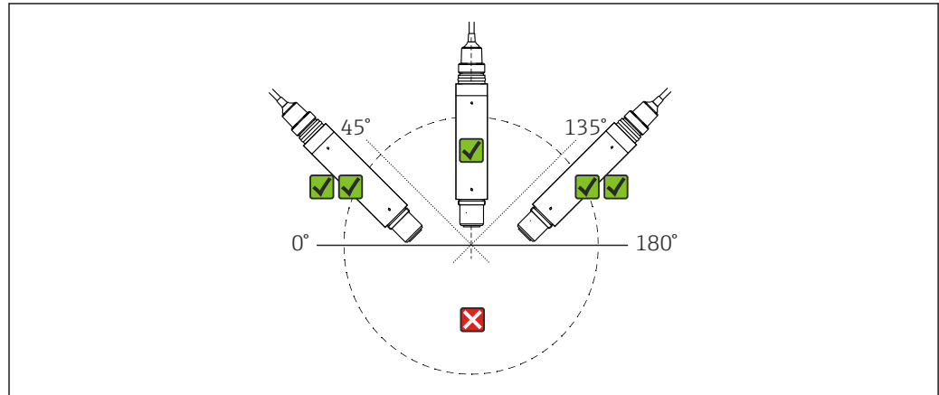
2 Installation angle
