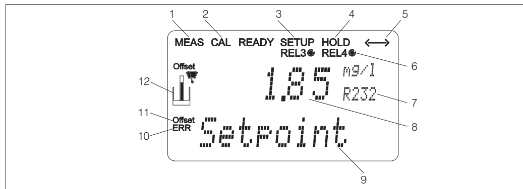
Fig. 22: LC display of transmitter
