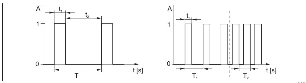
Fig. 35: Signal of a pulse-length modulated controller contact (left) and of a pulse-frequency modulated controller contact (right)
