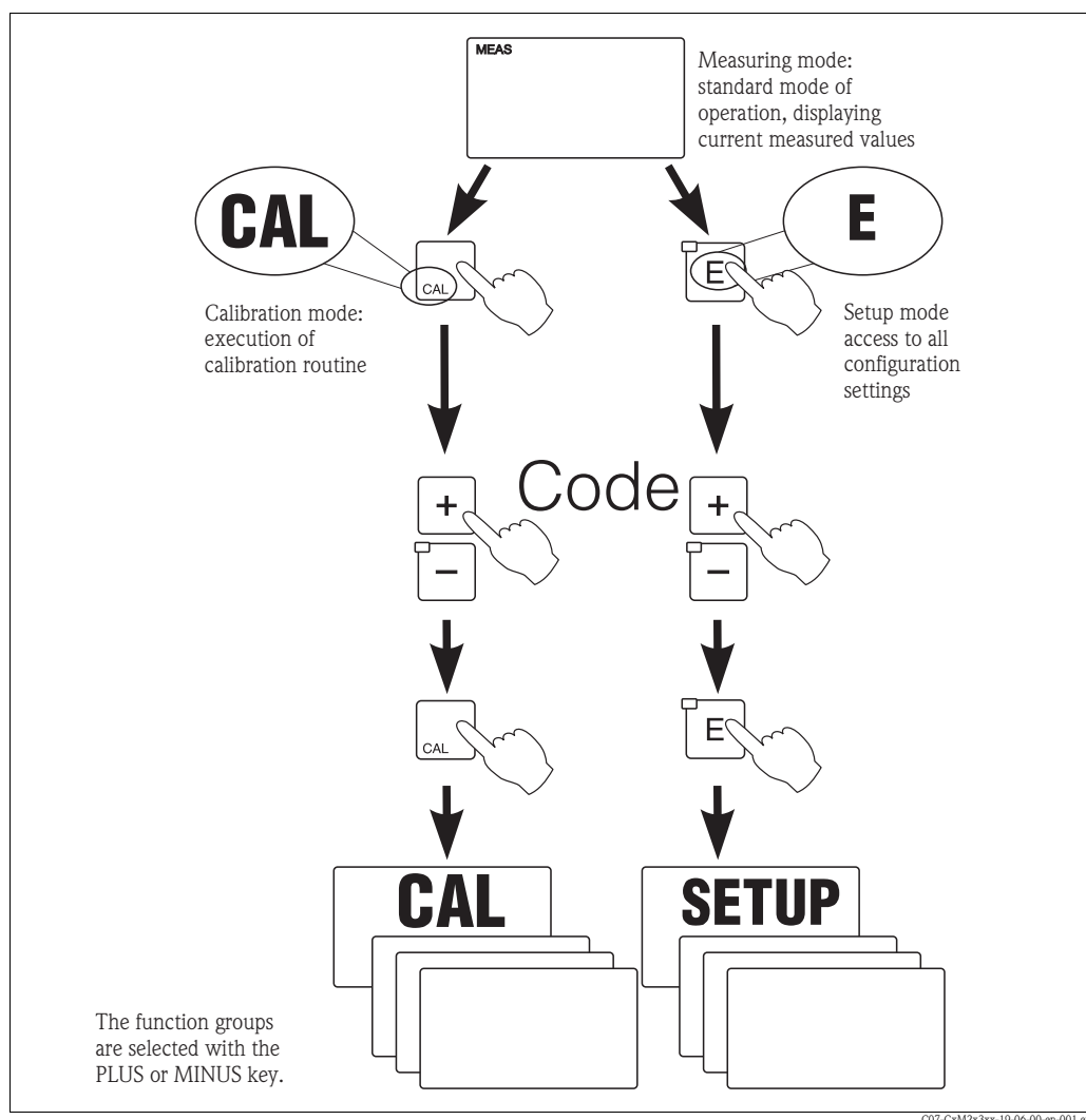
Fig. 24: Description of the possible operating modes
