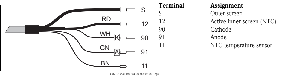
Fig. 14: Measuring cable CMK or CYK71
