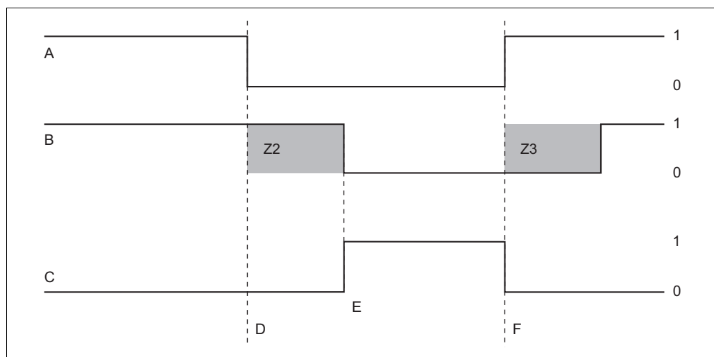
Fig. 28: Alarm signalling and dosing switch-off by the main stream
