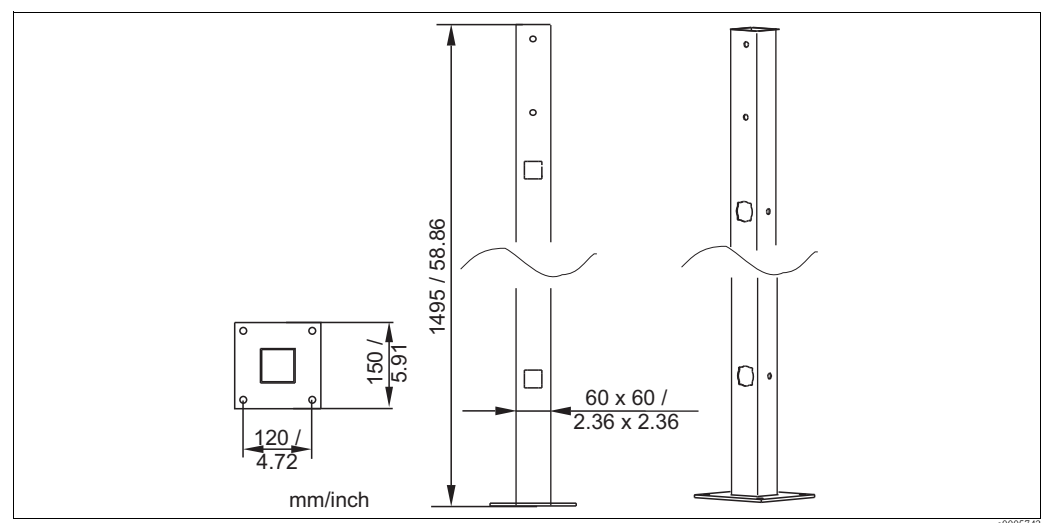
Fig. 40: Universal post
