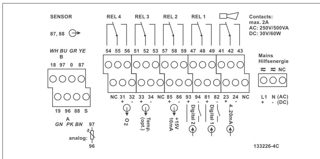
Fig. 17: Field instrument connection compartment sticker version WX/WS
