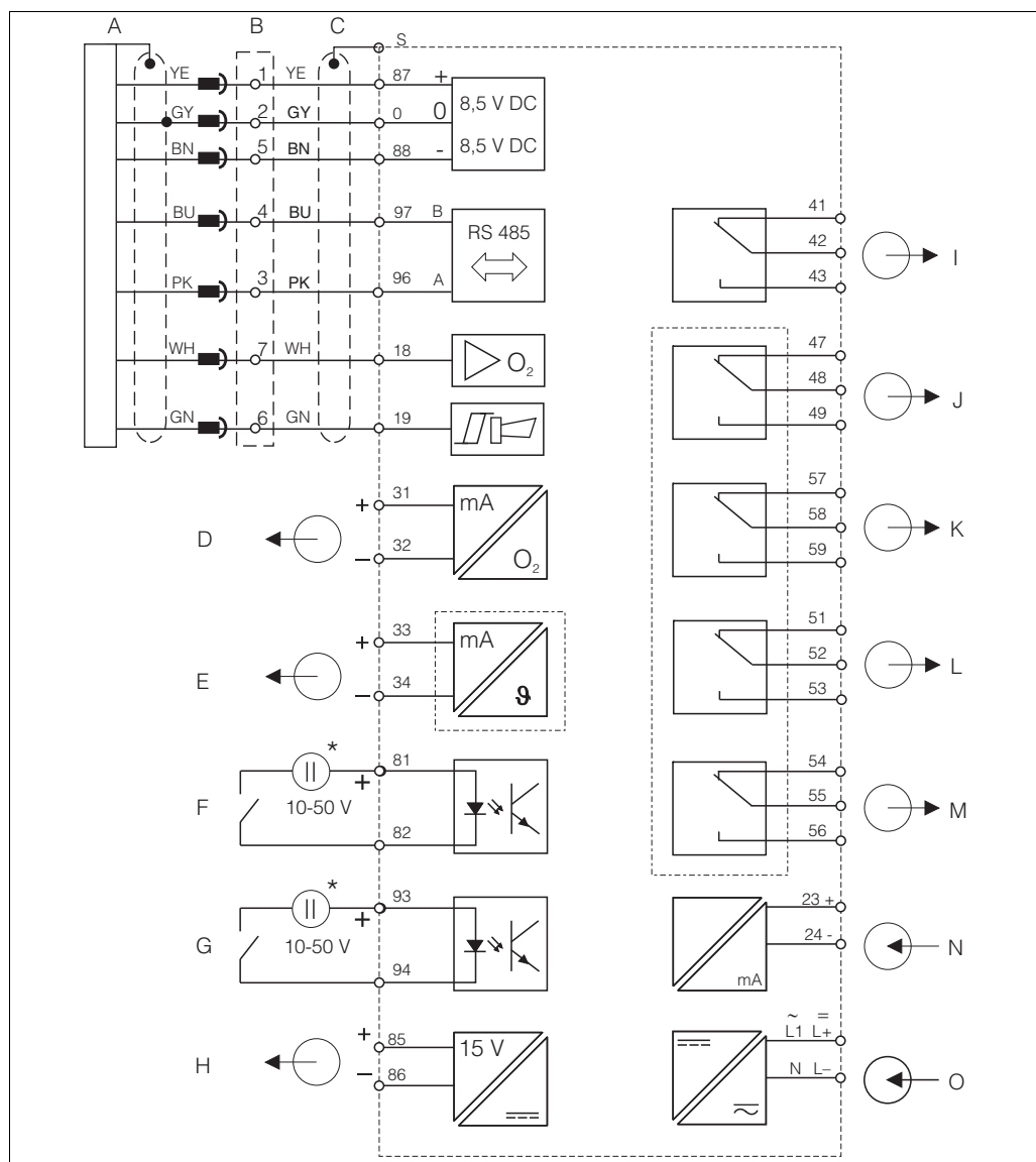
Fig. 16: Electrical connection of the transmitter version WX or WS
