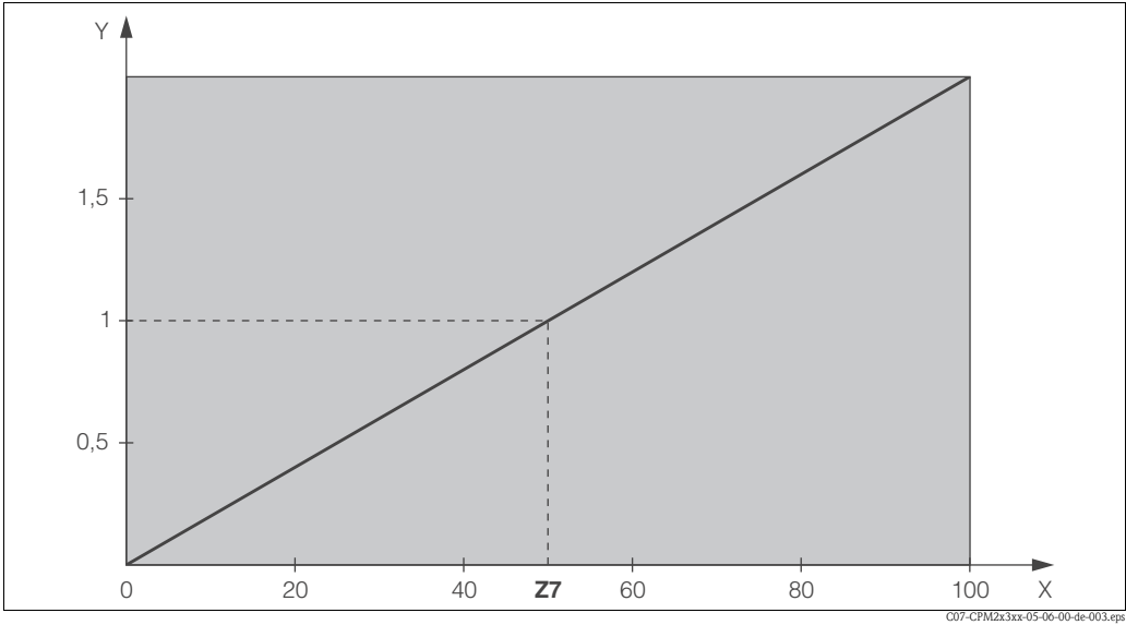
Fig. 30: Multiplying feedforward control Y Gain K_{infl} X Current input signal [%] Z7 Input value, when gain K_{infl} = 1
