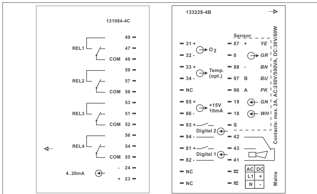
Fig. 18: Panel mounted instrument connection sticker
