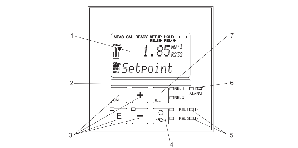
Fig. 23: Operating elements
