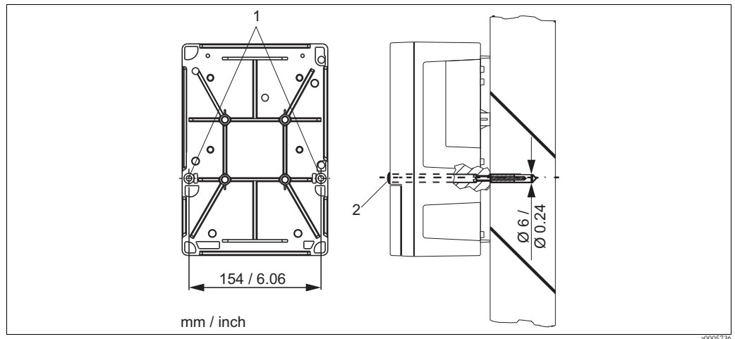
Fig. 7: Wall mounting field device
