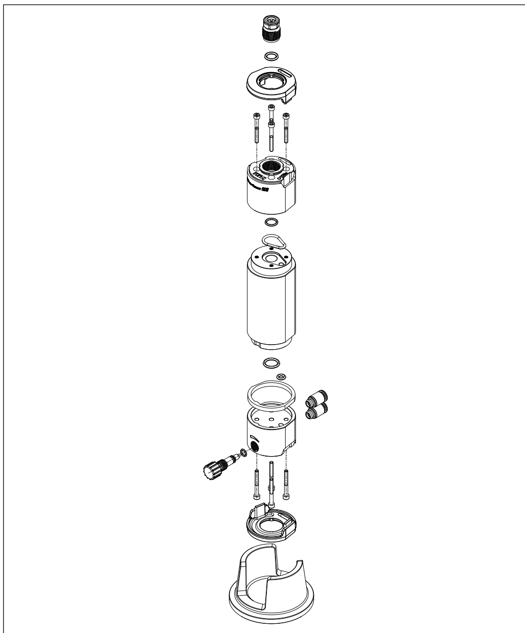
6 Exploded drawing with sealing rings
