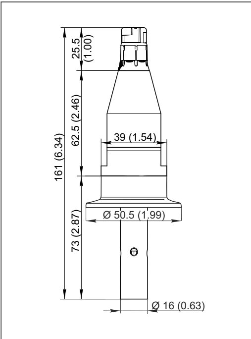
13 Version with Clamp
