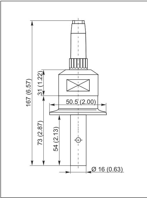
17 Plug-in head version with Clamp 1 1/2"
