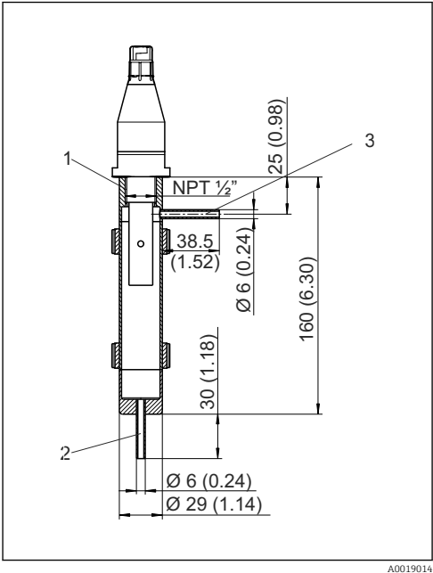
6 With NPT 1/2" thread in flow assembly 71042405, dimensions in mm (inch) 1 Sensor holder NPT 1/2" 2 Inlet 3 Outlet
