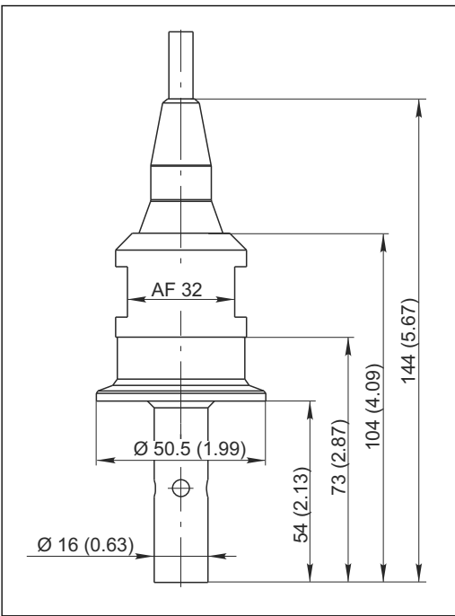
15 Fixed cable version with Clamp 1 1/2"
