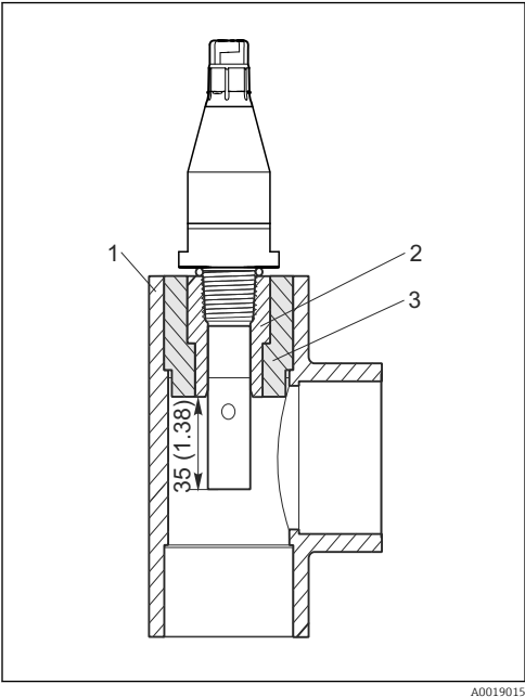
5 With NPT 1/2" thread in T-piece or cross fitting 1 T-piece or cross fitting (DN 32, 40 or 50) 2 Glue-in VC threaded coupling (NPT 1/2" for DN 20, see "Accessories") 3 Glue-in adapter coupling (for DN 32, 40, 50, see "Accessories")
