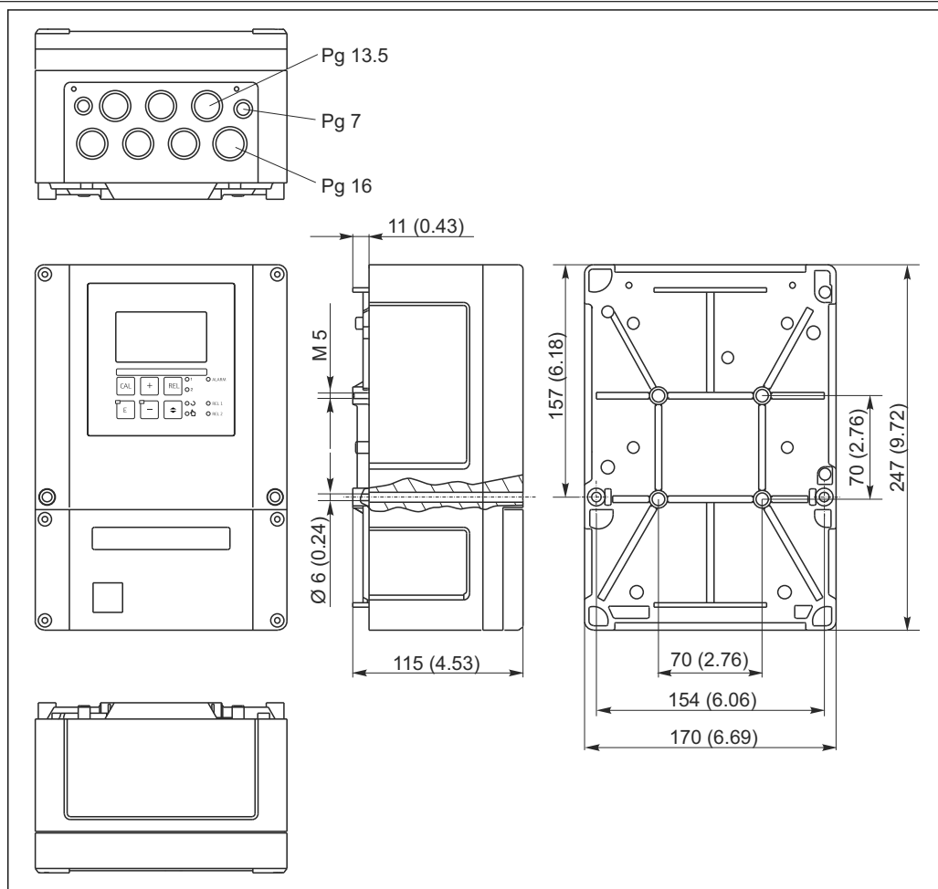
10 Field device: dimensions in mm (inch)
