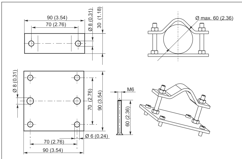
14 Dimensions in mm (inch)
