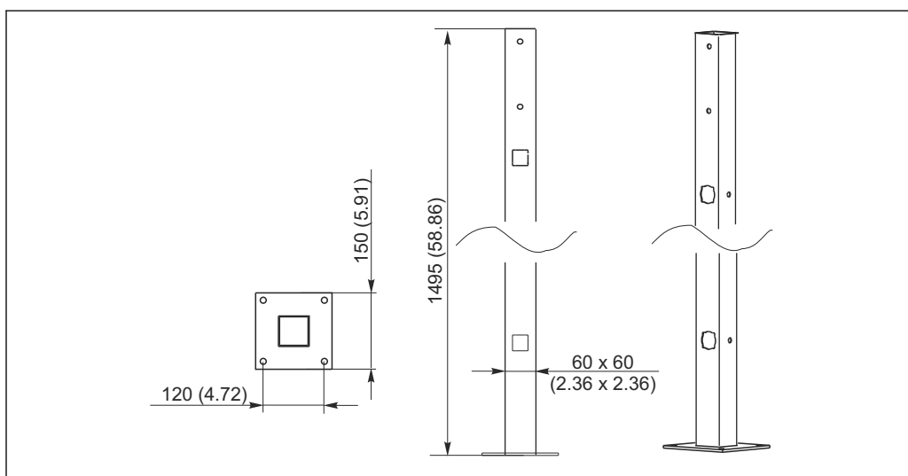
15 Dimensions in mm (inch)
