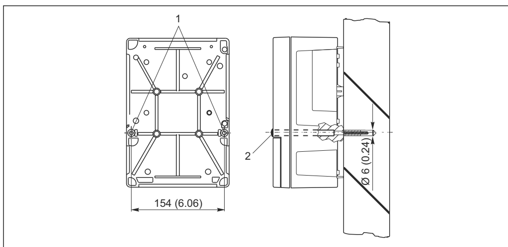
5 Field device wall mounting
