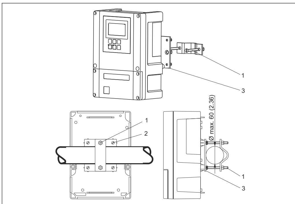
6 Field device on horizontal or vertical pipes
