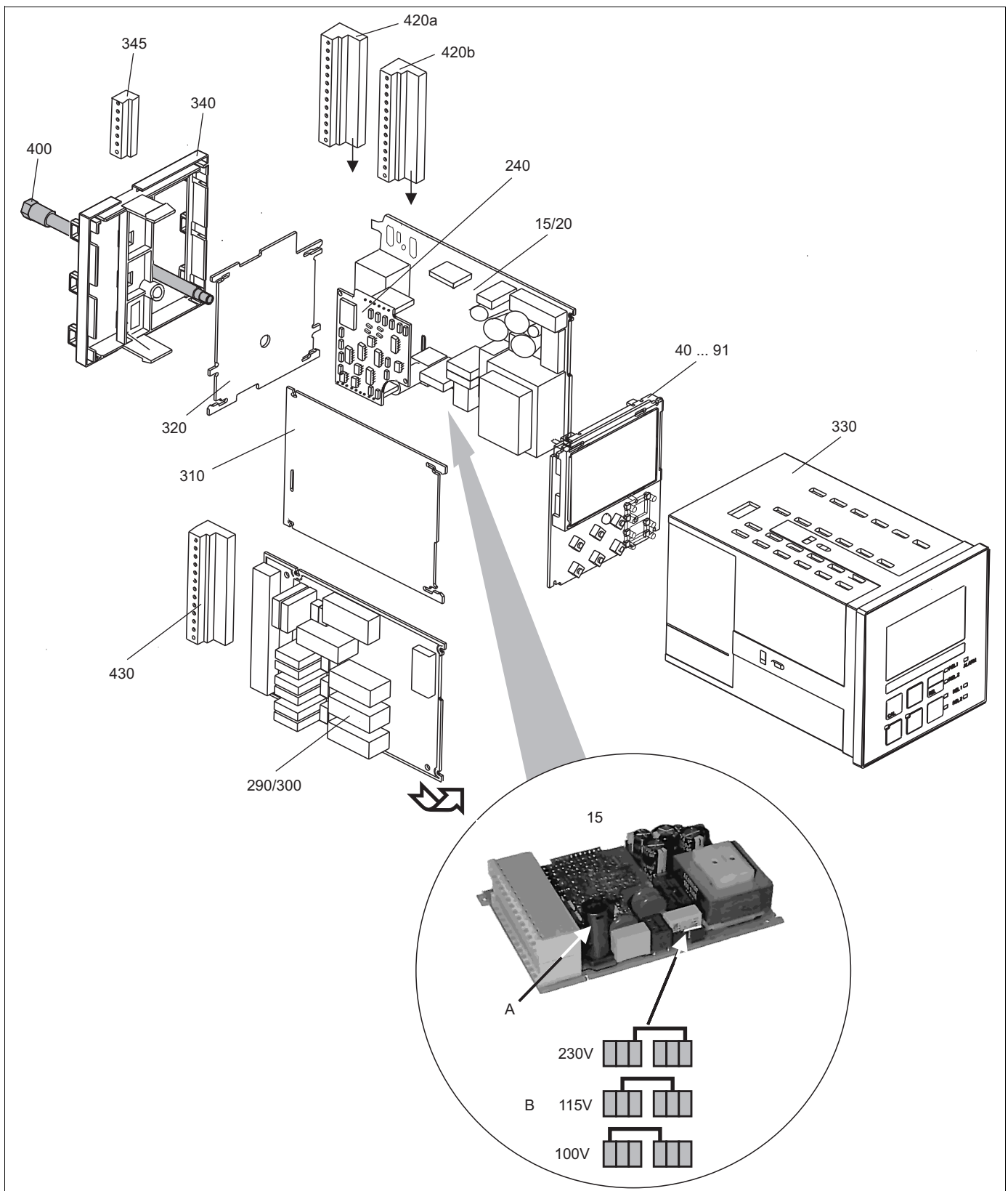
Fig. 44: Exploded view of panel mounted instrument
