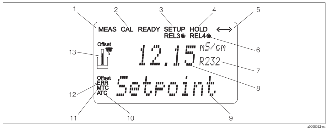
Fig. 18: LC display transmitter
