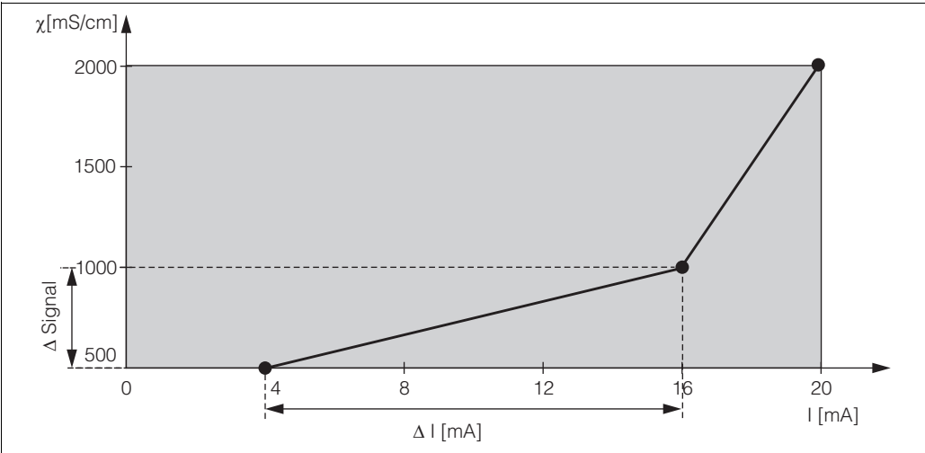
Fig. 29: User-defined current output characteristic (example)
