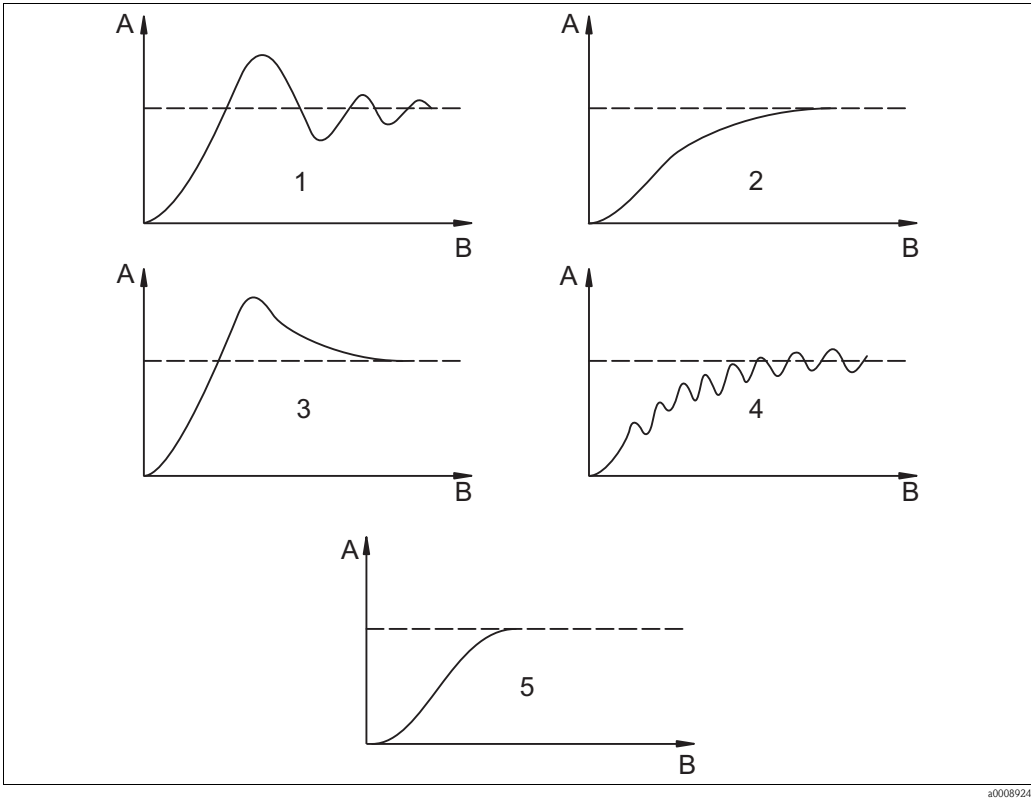
Fig. 33: Optimization of settings T_n and K_p
