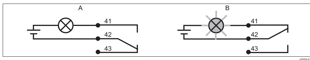
Fig. 17: Recommended fail-safe switching for the alarm contact
