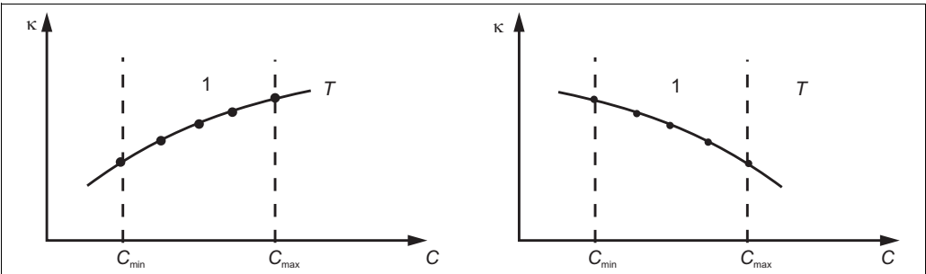
Fig. 39: Measured data for a constant process temperature (example) κ Constant temperature C Concentration T Constant temperature 1 Measuring range
