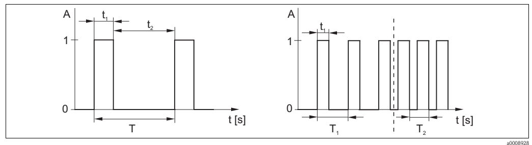
Fig. 34: Signal of a pulse-length modulated controller contact (left) and of a pulse-frequency modulated controller contact (right)
