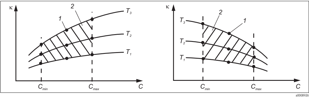
Fig. 38: Measured data for variable process temperatures (example) κ Conductivity C Concentration T Temperature 1 Measuring point 2 Measuring range
