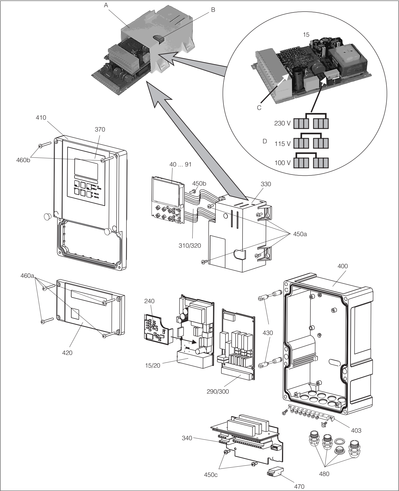
Fig. 45: Exploded drawing of field instrument
