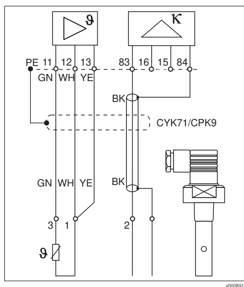
Fig. 15: Connection of conductive sensors
