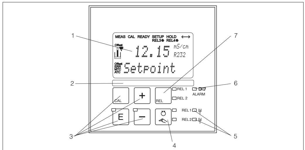
Fig. 19: Operating elements
