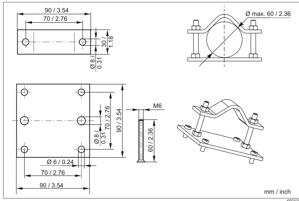
Fig. 43: Post mounting kit
