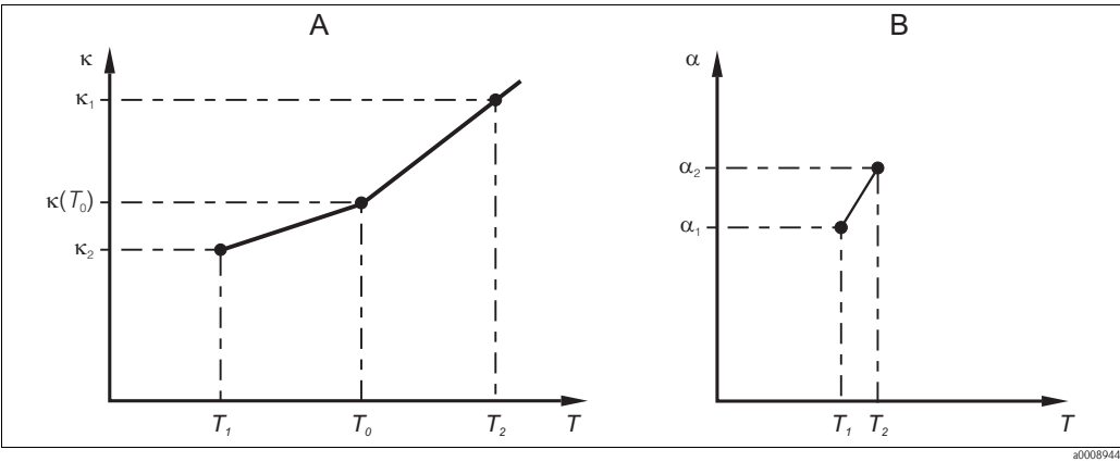
Fig. 26: Determination of temperatur coefficient
