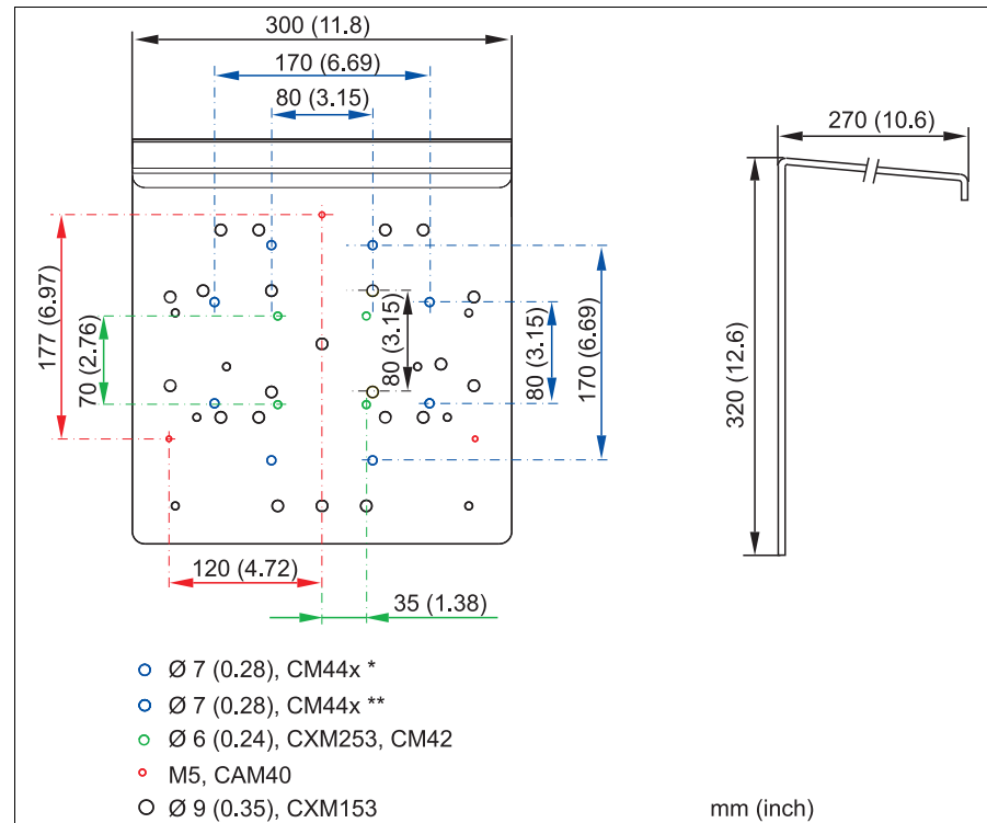
Fig. 41: Weather protection cover for field devices
