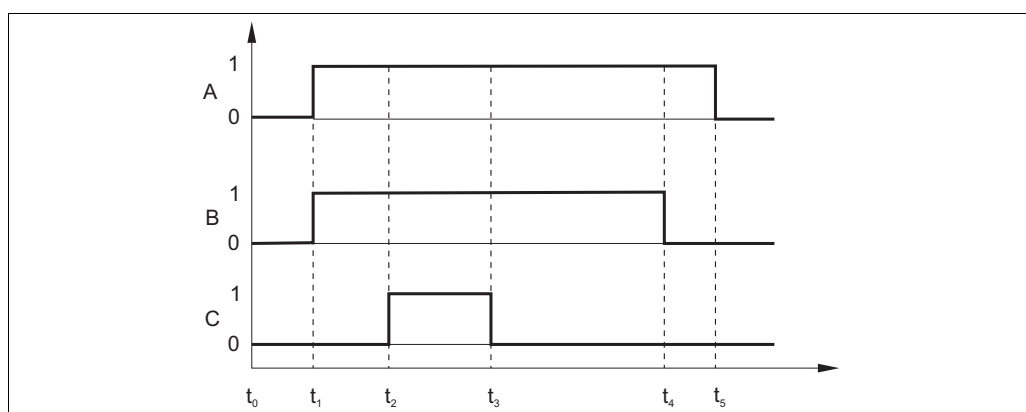
Fig. 37: Sequence of a cleaning cycle
