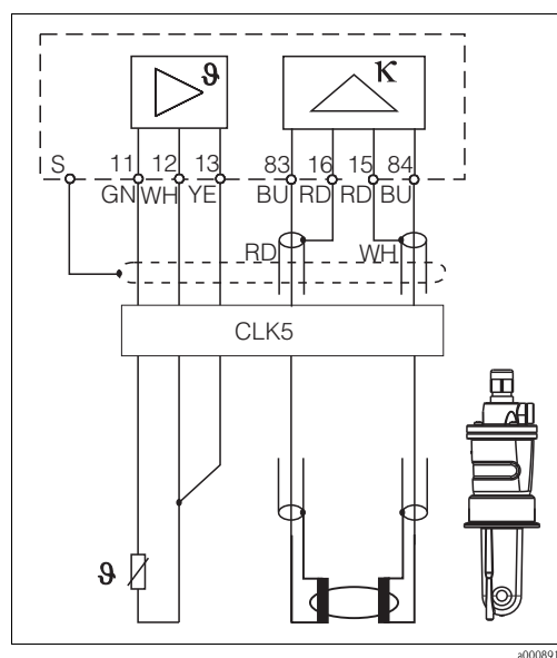
Fig. 16: Connection of inductive sensors
