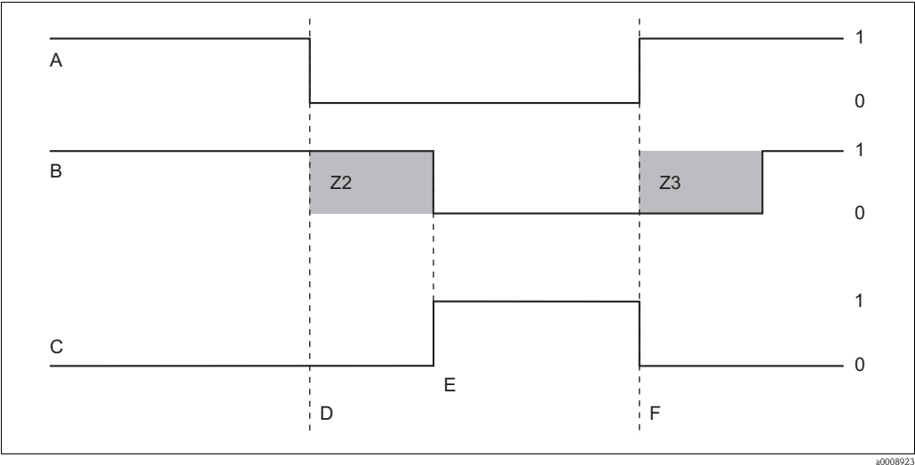
Fig. 27: Alarm signalling and dosing switch-off by the main stream A Flow in main stream F Flow restoration B Relay contacts of PID controller Z2 Delay for controller switch-off, see field Z2 C Alarm relay Z3 Delay for controller switch-on, see field Z3 D Flow below switch-off limit Z4 or flow failure 0 Off E Flow alarm 1 On
