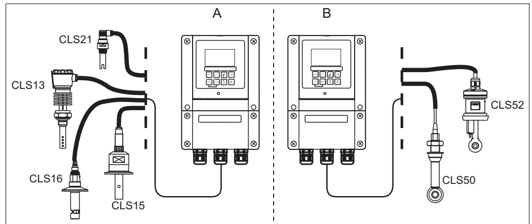
Measuring system
