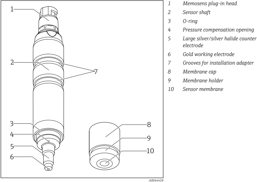
1 Sensor structure
