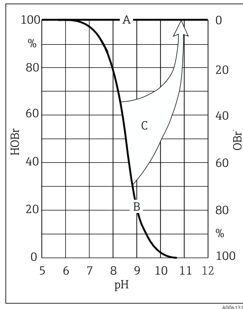
2 Principle of pH compensation
