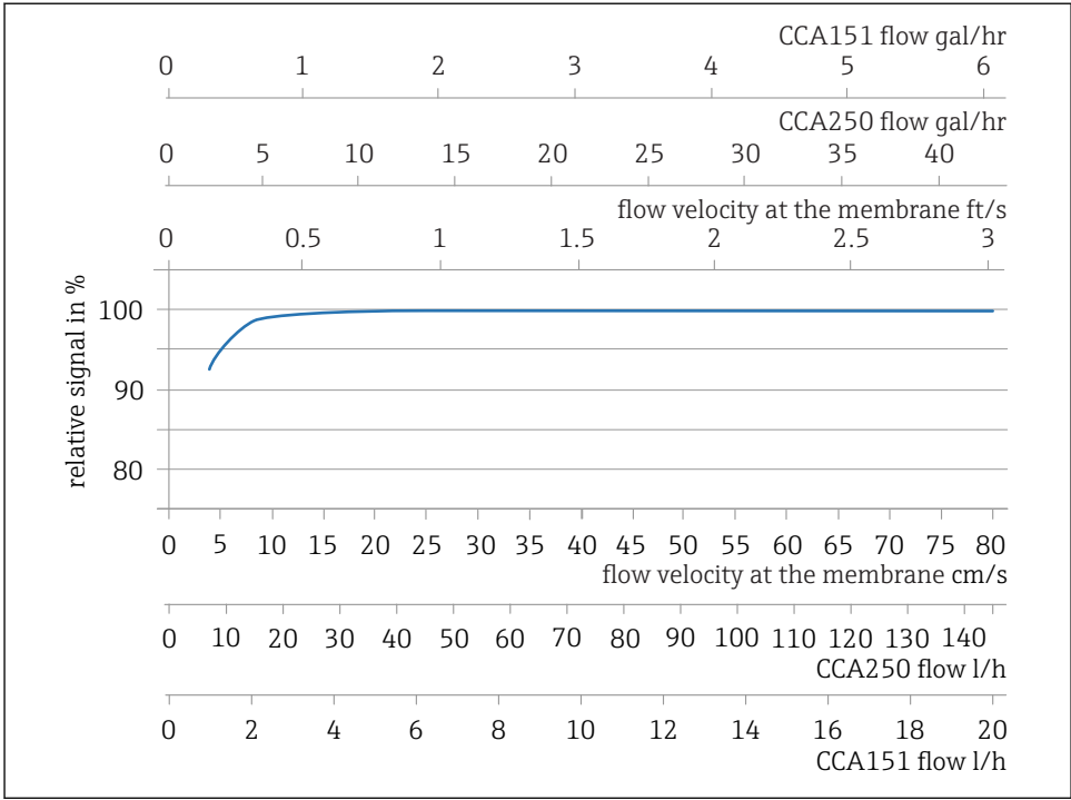
3 Correlation between slope of electrode and flow velocity at the membrane/volume flow in assembly
