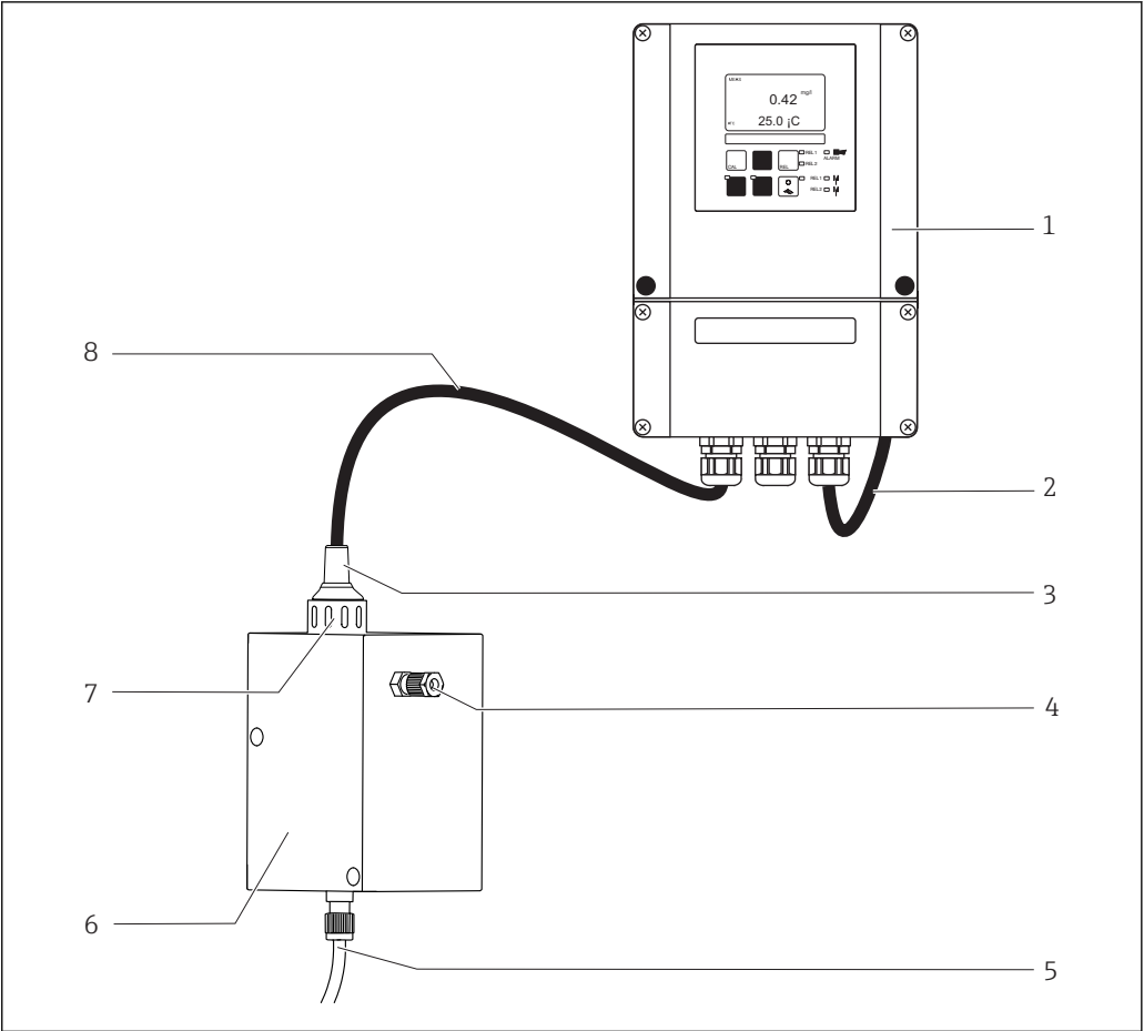
1 Example of a measuring system
