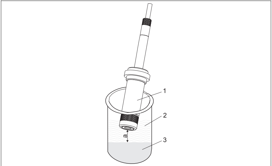
Fig. 8: Reconditioning of the sensor above aqueous chlorine dioxide solution
