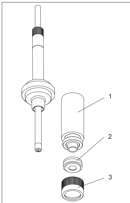
Fig. 7: Membrane replacement
