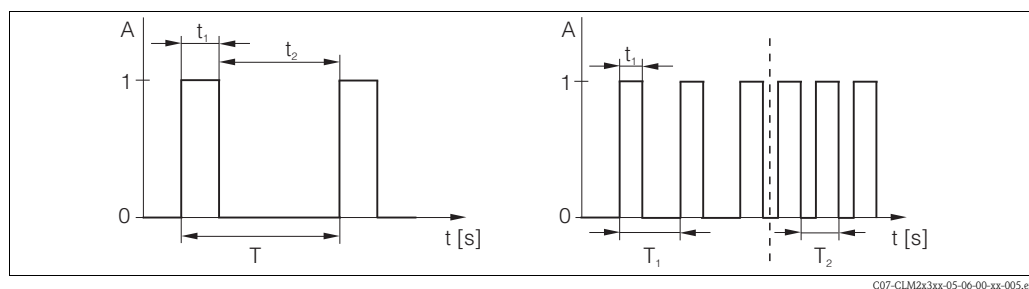
Fig. 41: Signal of a pulse-length modulated controller contact (left) and of a pulse-frequency modulated controller contact (right)
