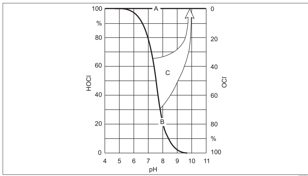
Fig. 33: Schematic diagram of pH compensation
