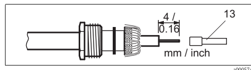
Fig. 20: Terminating the pH connecting cable for mounting the BNC elbow plug
