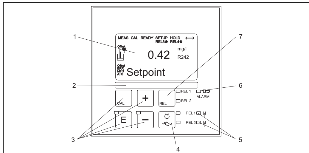
Fig. 27: Operating elements
