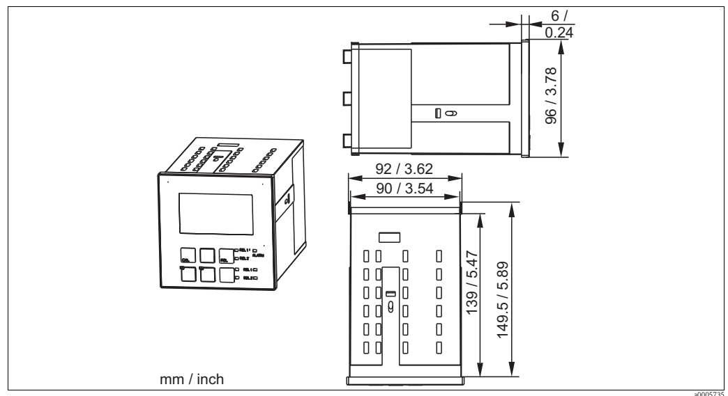
Fig. 7: Panel-mounted instrument
