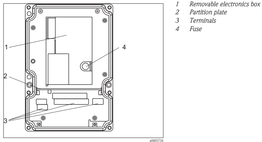
Fig. 6: View into the field housing
