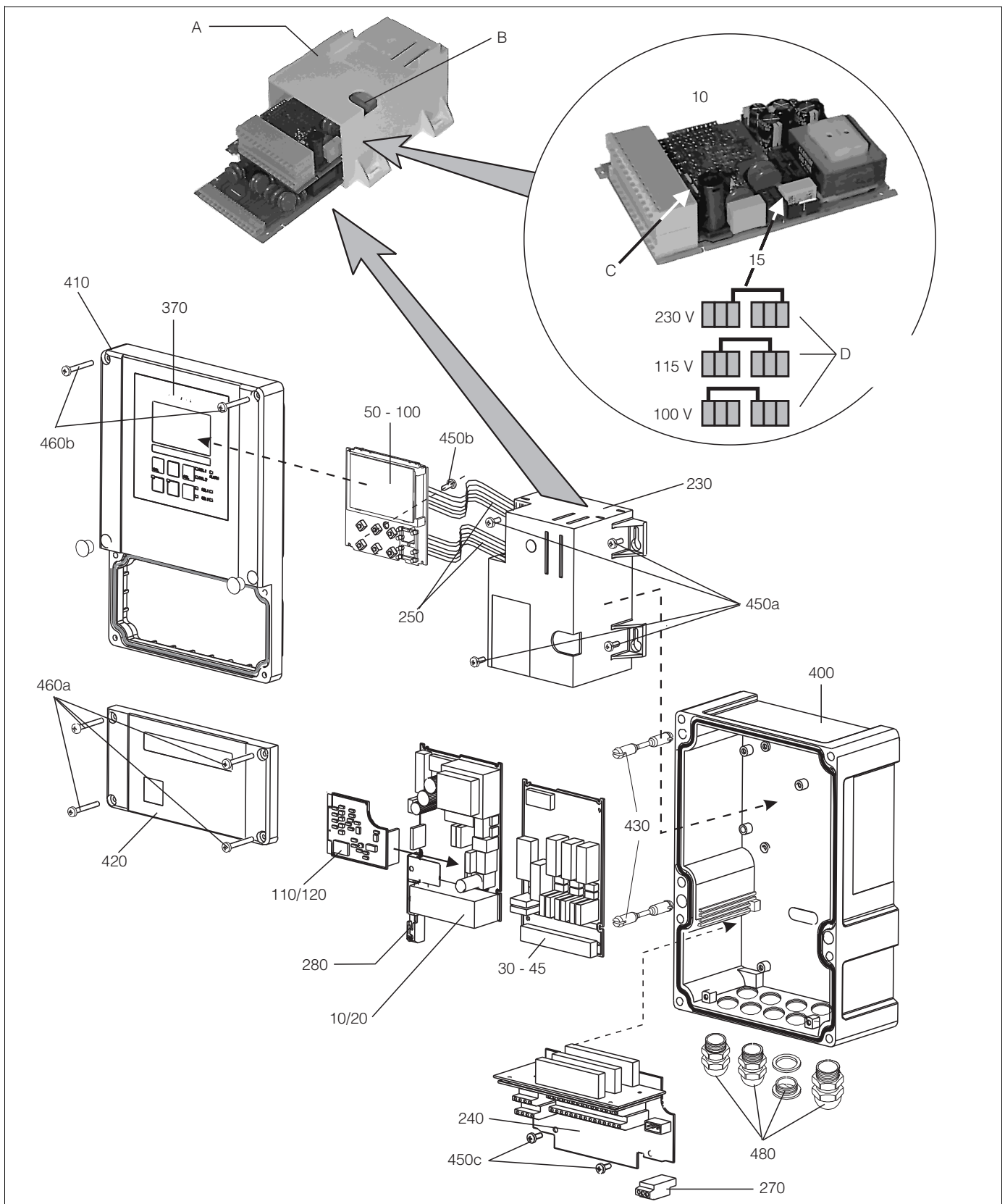
Fig. 51: Exploded view drawing of field instrument
