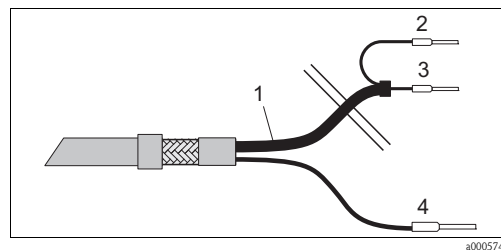
Fig. 18: Cable CPK1: device connection
