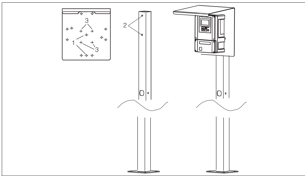
Fig. 10: Mounting field device with universal posts and weather protection cover
