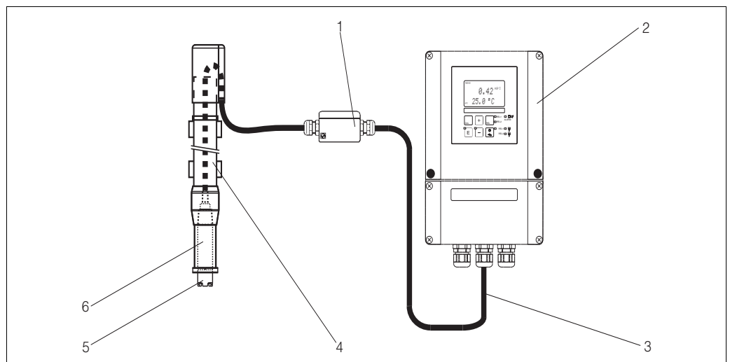
Fig. 4: Measuring system with immersion assembly (example)
