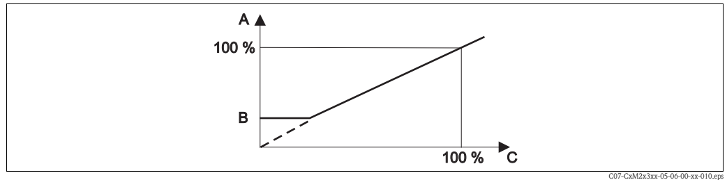
Fig. 39: Control characteristic PID controller with basic load dosing
