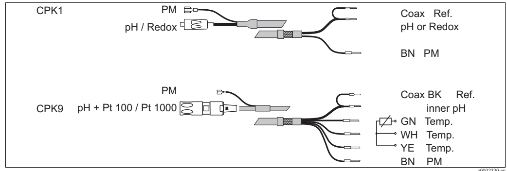
Fig. 17: Connection of the pH or ORP sensor to the field instrument with the cables CPK1 or CPK9
