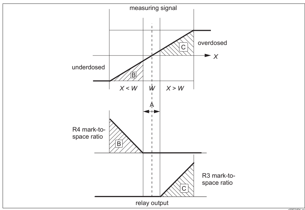
Fig. 45: Function of the three-point step controller
