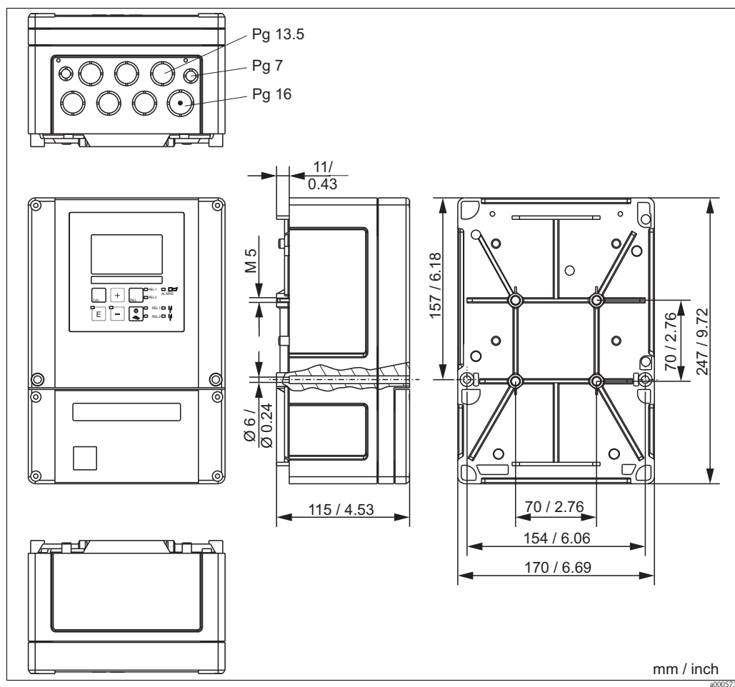
Fig. 5: Field instrument
