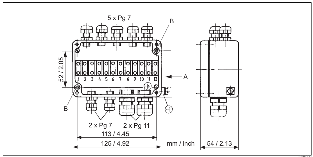
Fig. 22: VBC junction box with grounding point
