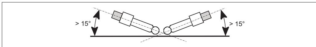
Fig. 46: Permitted installation angle of glass electrodes
