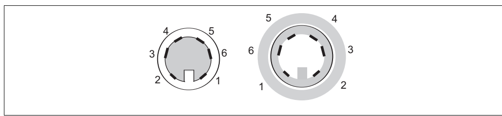
Fig. 16: TOP68 plug connection; pin assignment of plug, male and female (shown from contact side)
