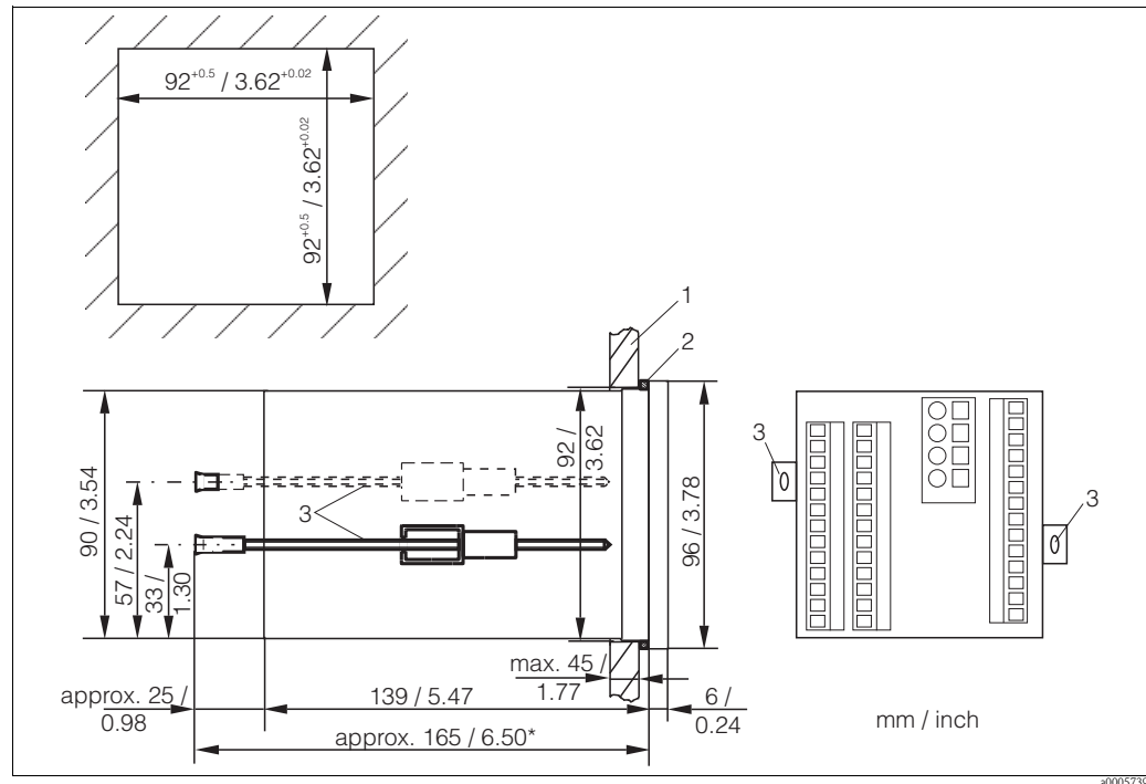
Fig. 11: Securing the panel-mounted instrument
