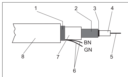
Fig. 23: CMK cable
