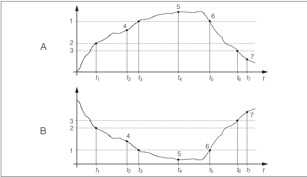
Fig. 38: Illustration of the alarm and limit value functions A Switch-on point > switch-off point: Max. function 1 Alarm threshold 5 Alarm ON B Switch-on point < switch-off point: Min. function 2 Switch-on point 6 Alarm OFF 3 Switch-off point 7 Contact OFF 4 Contact ON
