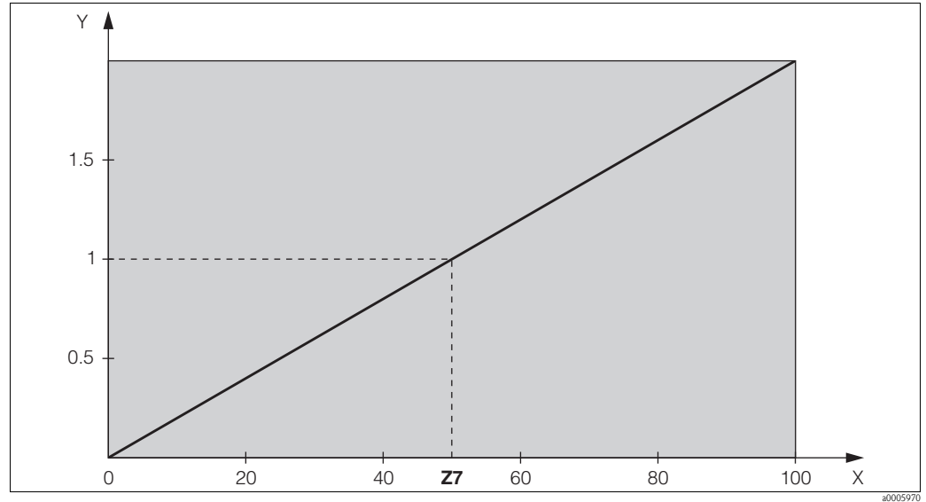
Fig. 36: Multiplying feedforward control
