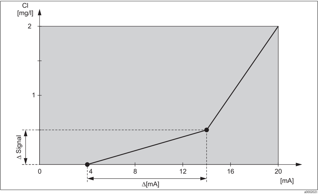
Fig. 37: User-defined current output characteristic (example)
