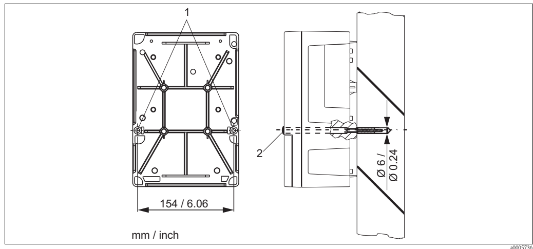
Fig. 8: Wall mounting field device
