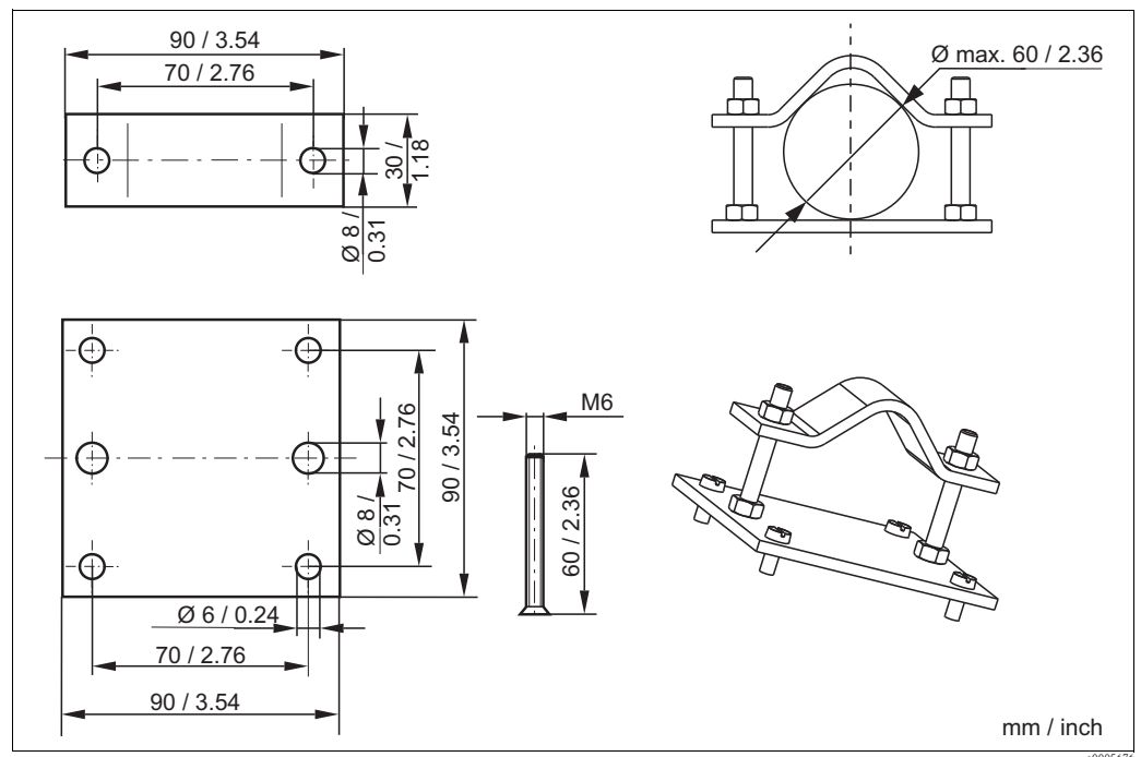
Fig. 49: Post mounting kit
