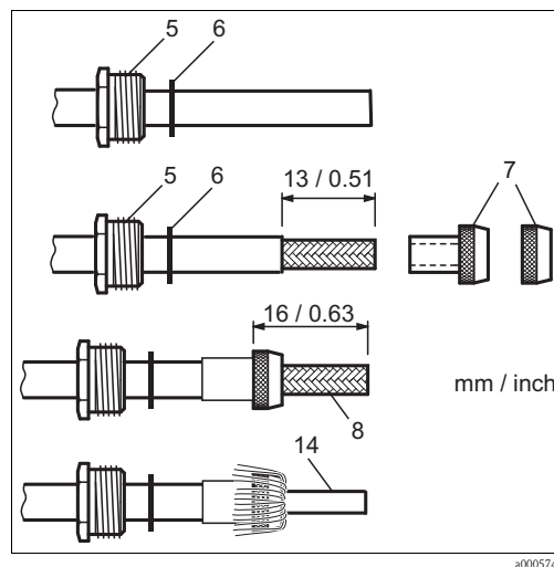
Fig. 19: Terminating the pH connecting cable for mounting the BNC elbow plug
