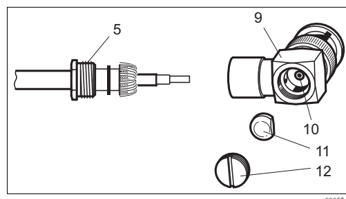
Fig. 21: Mounting the pH connecting cable in the BNC elbow plug
